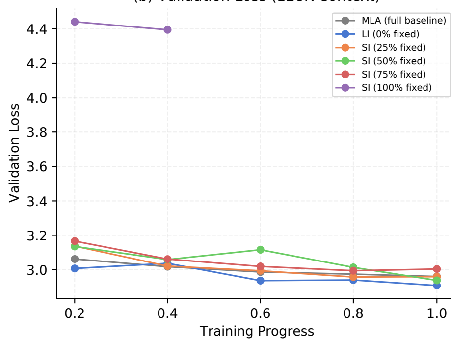
(b) Validation Loss (128K Context)
