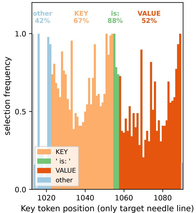
(b) Zoom-in: per-token selection frequency within the target needle line
