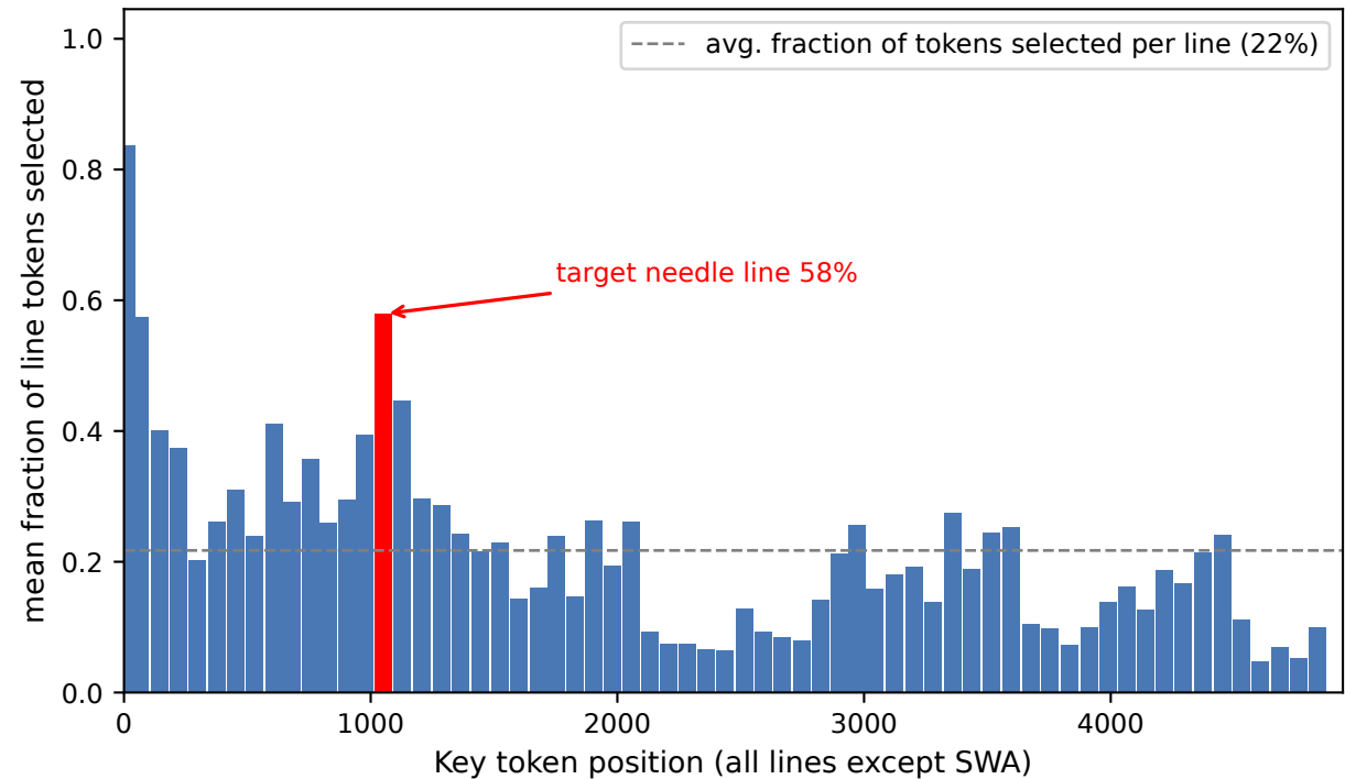
(a) Per-line selection density: indexer concentrates budget on the needle line (averaged over the question tokens)
