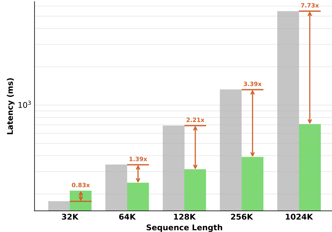
Total (Fwd + Bwd)
