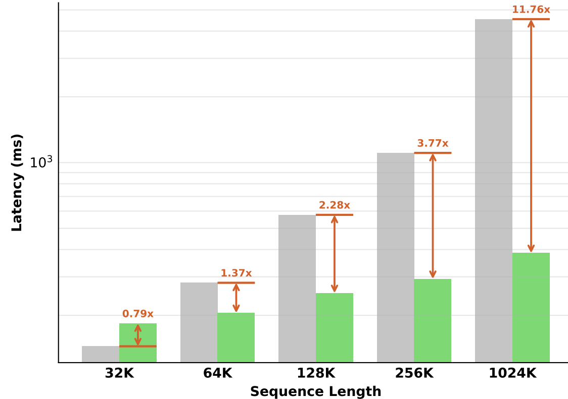
Backward
