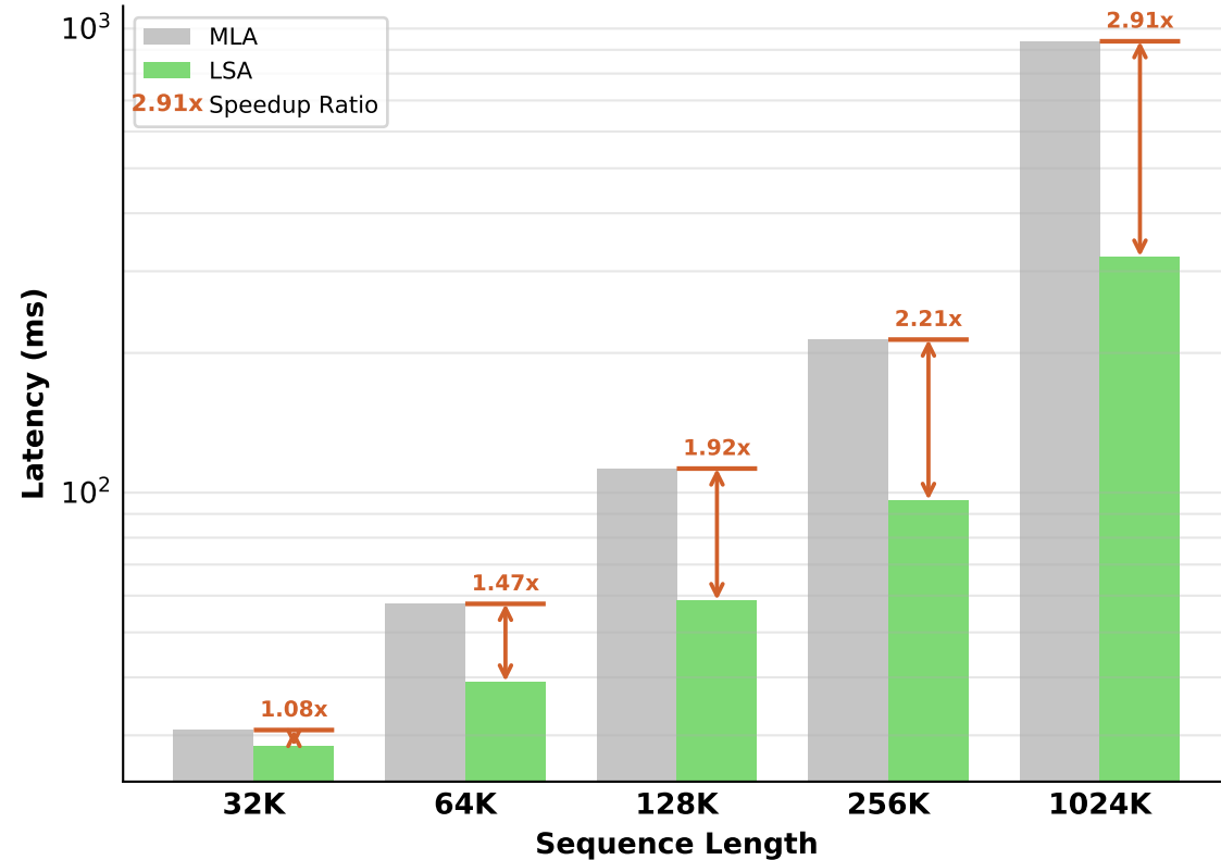
Forward
