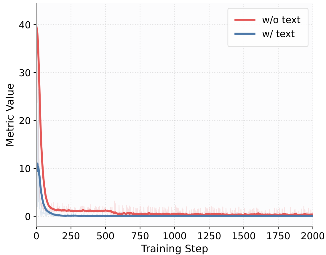
Training Loss
