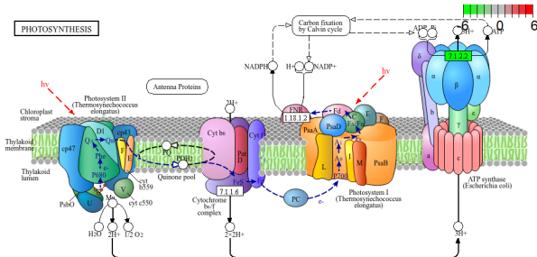
Photosystem II
