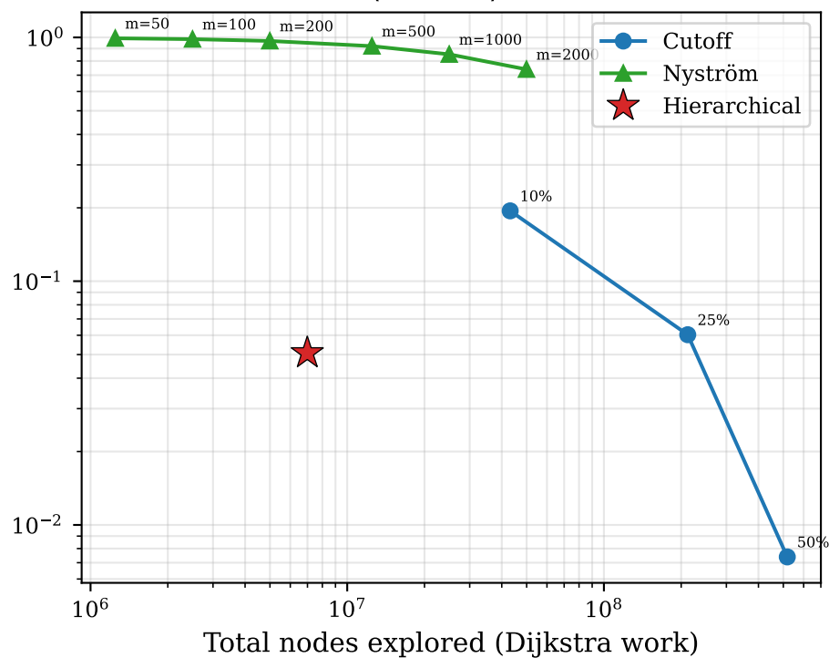
Error vs. Computation Time (n = 24,964)
