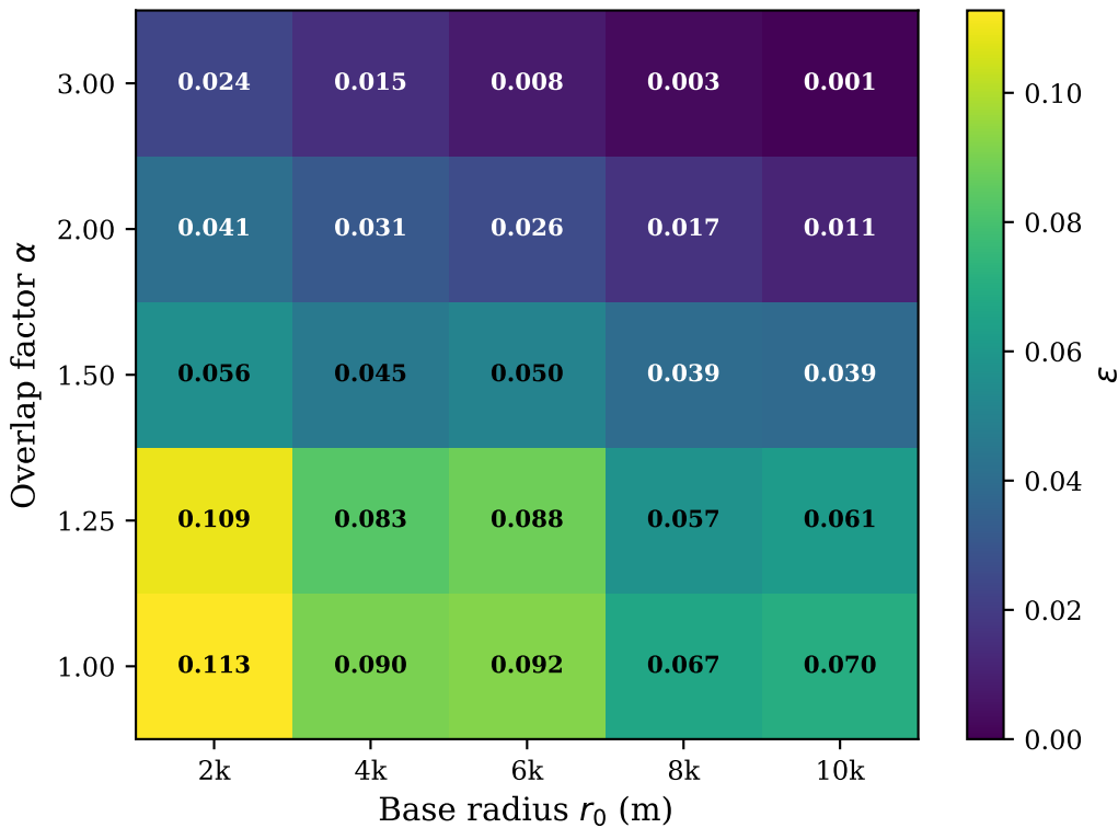
Relative RMSE — (c + 2000)^{-1.5} on 20 \times 20 grid
