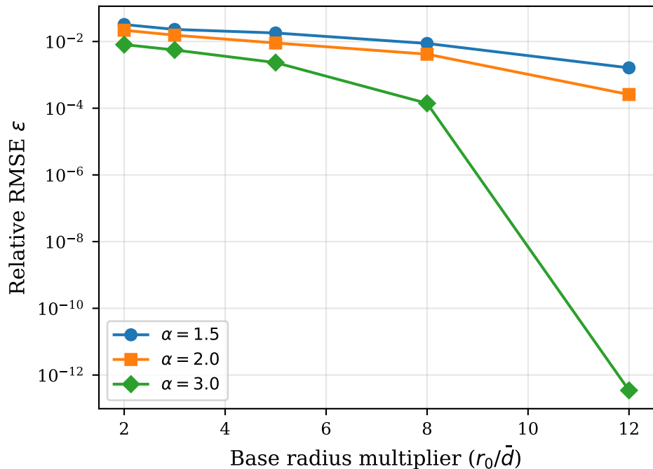
(b) Error vs. base radius ( n=2000 )
