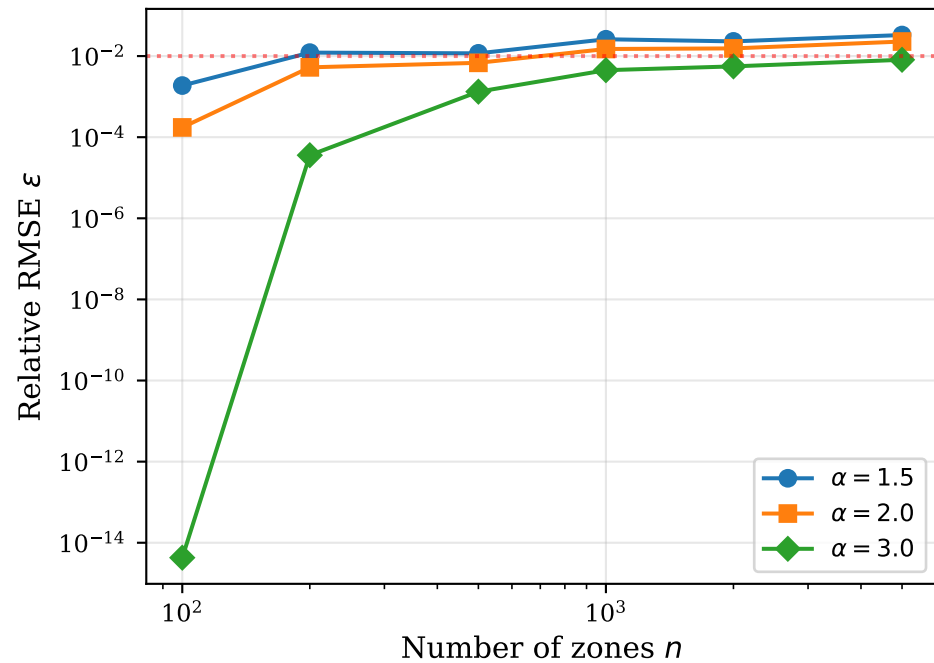
(a) Error with tuned r_0 = 3 \times edge length
