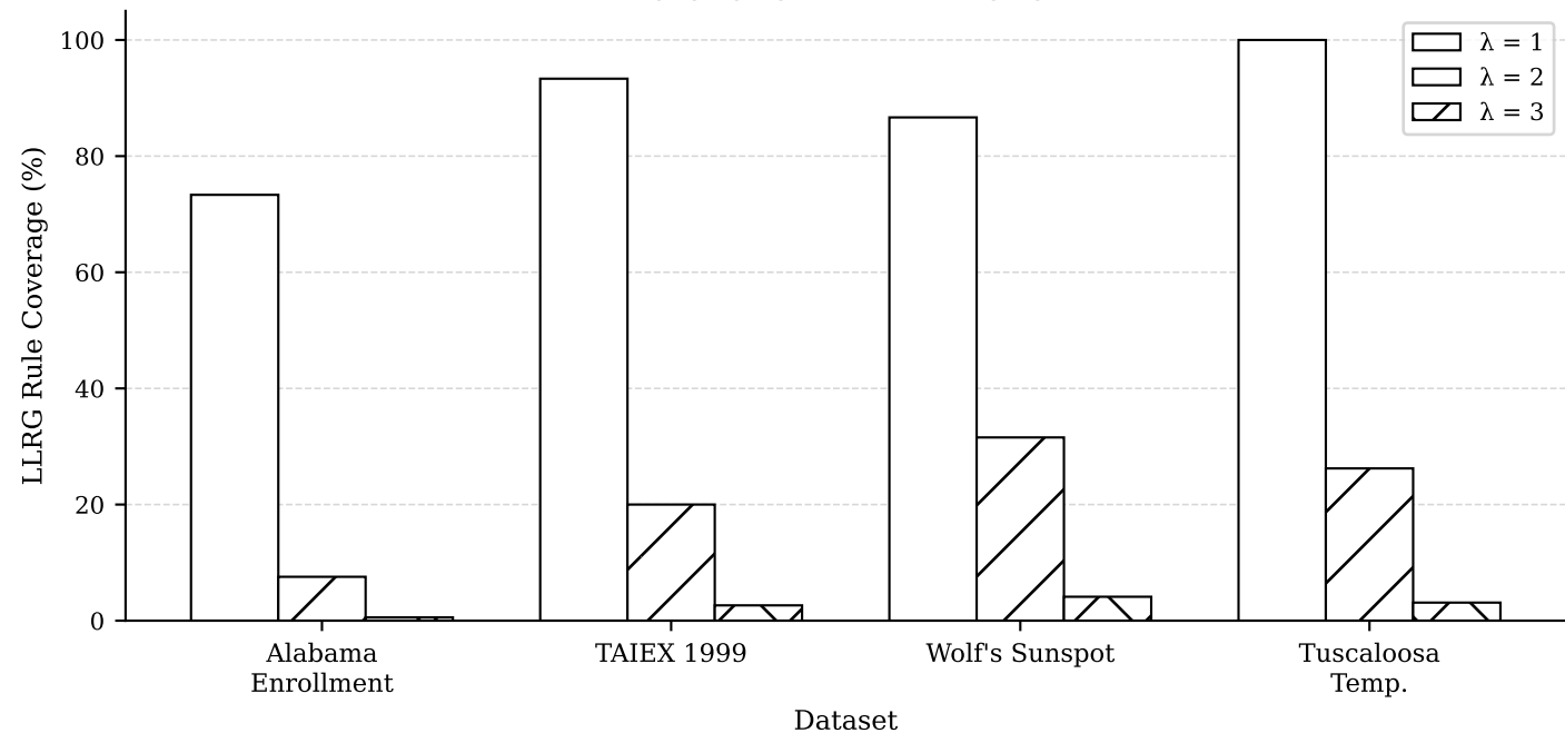
Rule Coverage Ratio vs. Forecasting Order (Coverage = |R| / |W|^\lambda \times 100\% , |W| = 15 , k = 2 )
