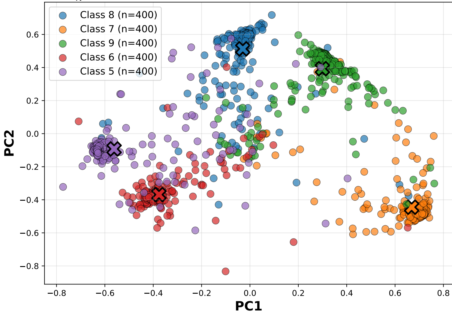
U_N^{hl} : Rare Class Embeddings (Avg Intra-dist=0.112)
