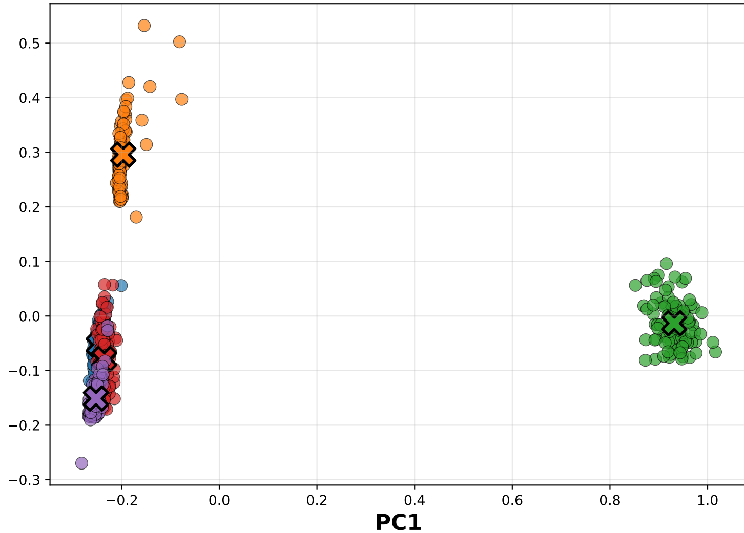
U_N : Rare Class Embeddings (Avg Intra-dist=0.039)
