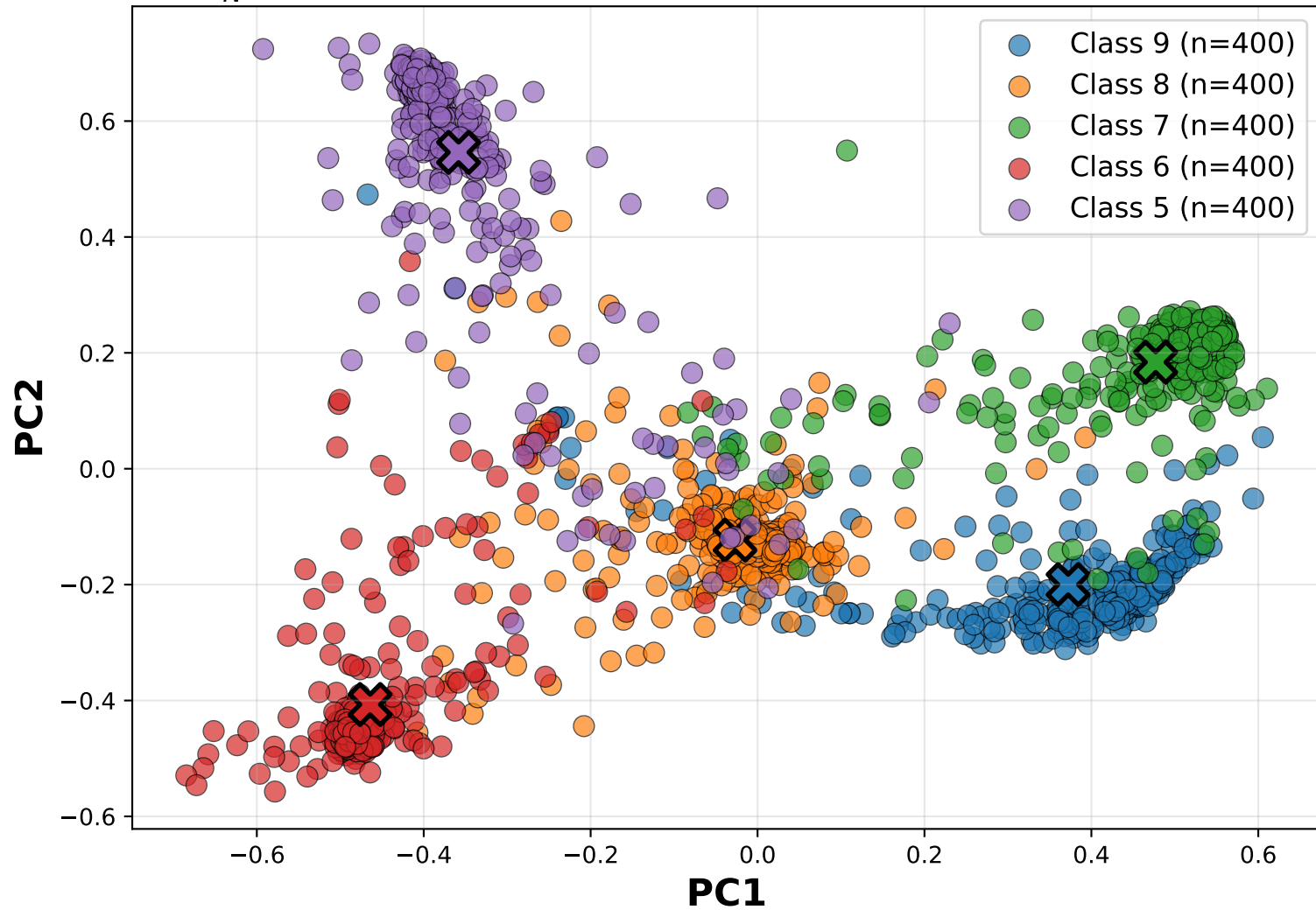
U_N^{hl} : Rare Class Embeddings (Avg Intra-dist=0.117)
