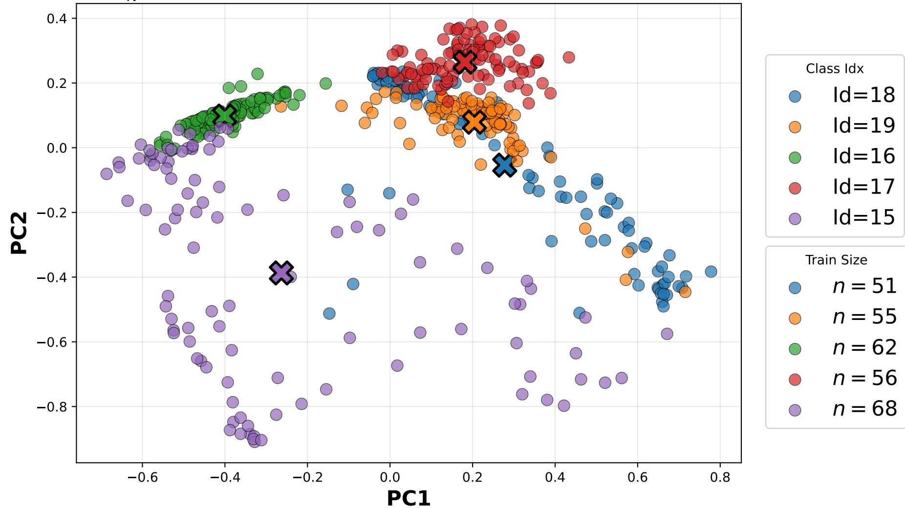
U_N^h : Rare Class Embeddings (Avg Intra-dist=0.217)
