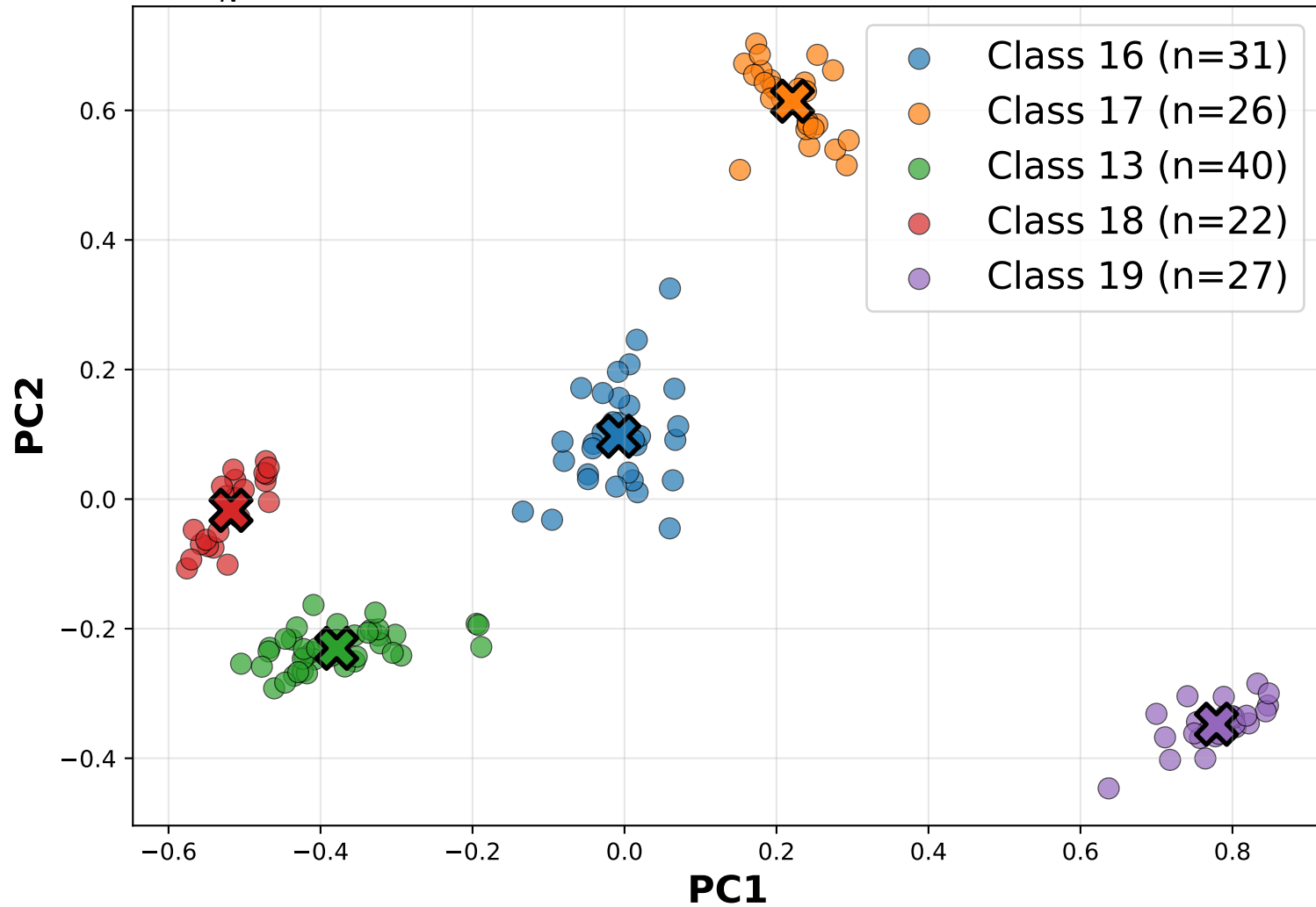
U_N^h : Rare Class Embeddings (Avg Intra-dist=0.063)
