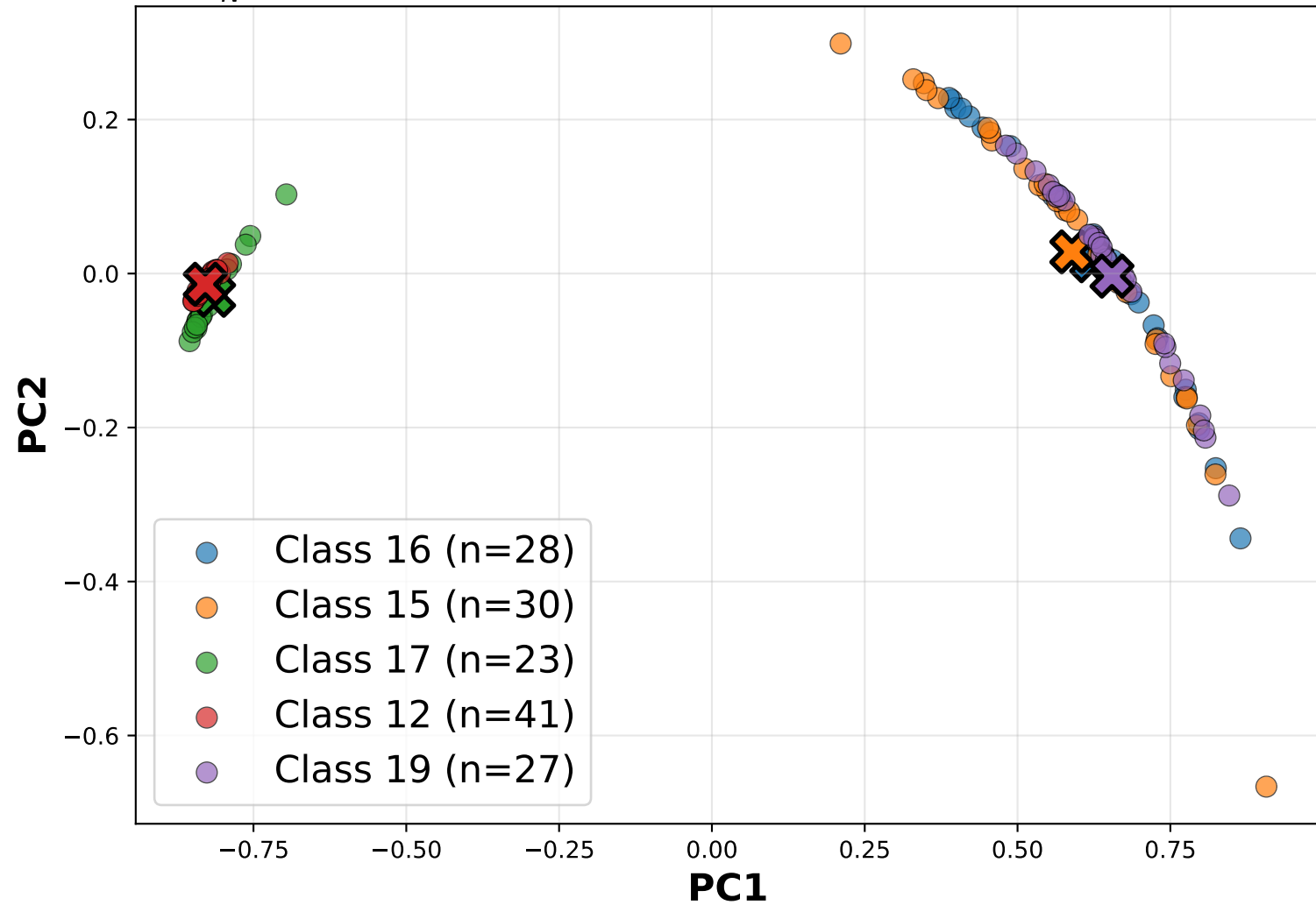
U_N^h : Rare Class Embeddings (Avg Intra-dist=0.112)
