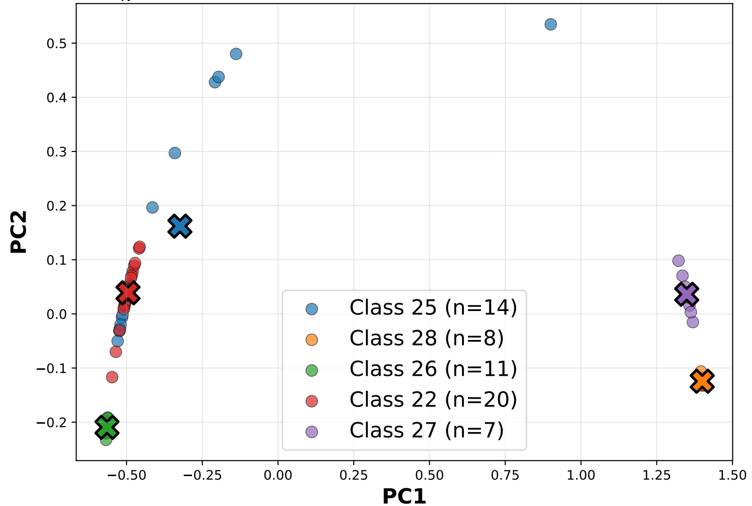
U_N^h : Rare Class Embeddings (Avg Intra-dist=0.085)
