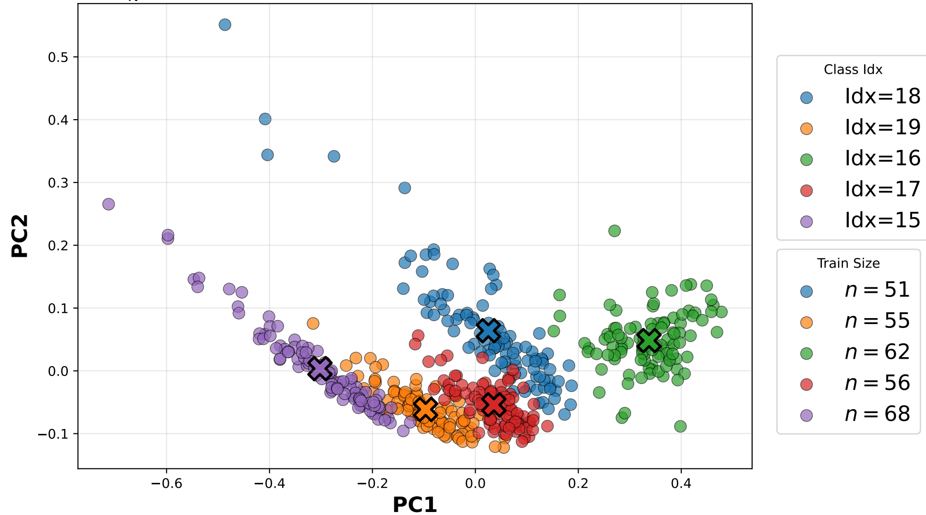
U_N^h : Rare Class Embeddings (Avg Intra-dist=0.081)
