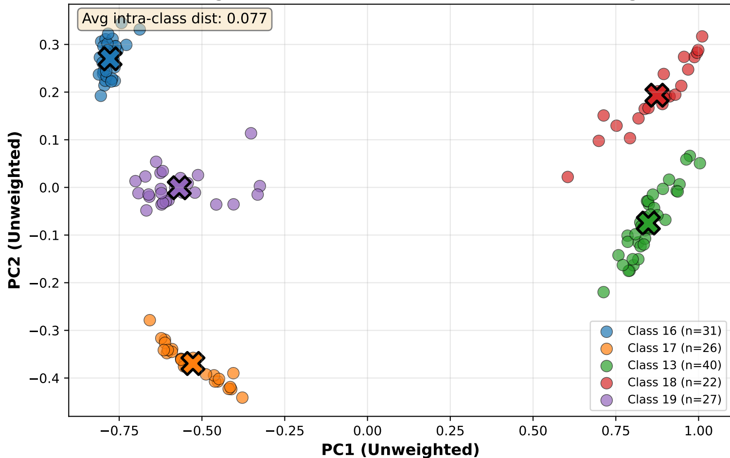
Unweighted U-Statistics: Rare Class Embeddings
