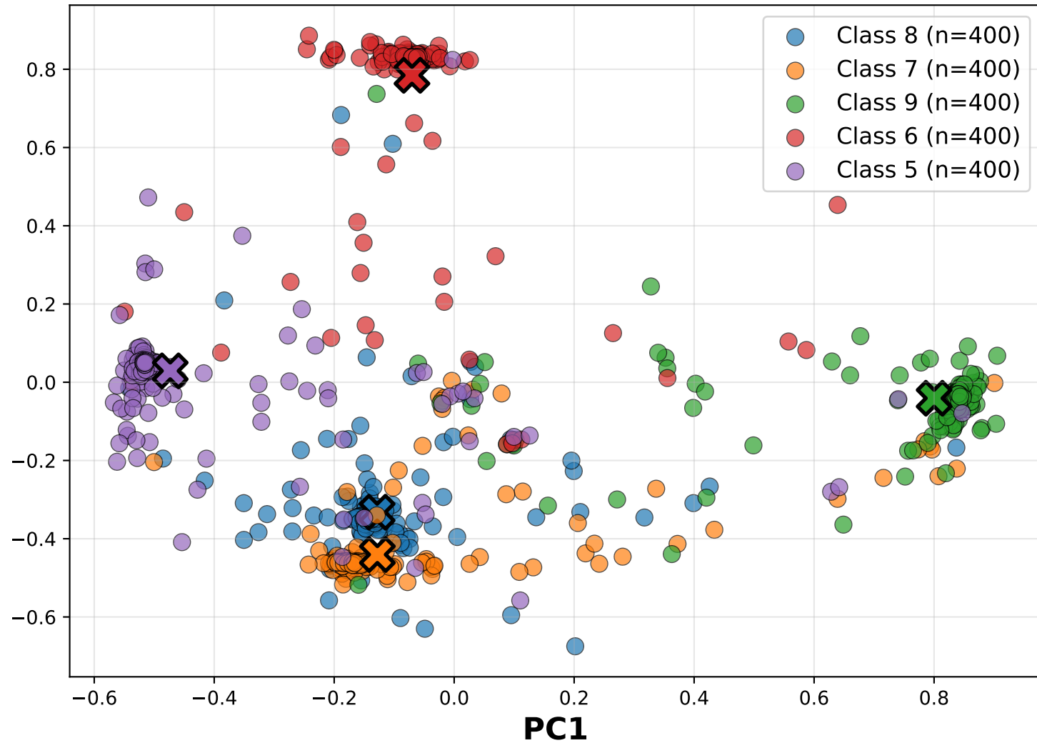
U_N : Rare Class Embeddings (Avg Intra-dist=0.088)
