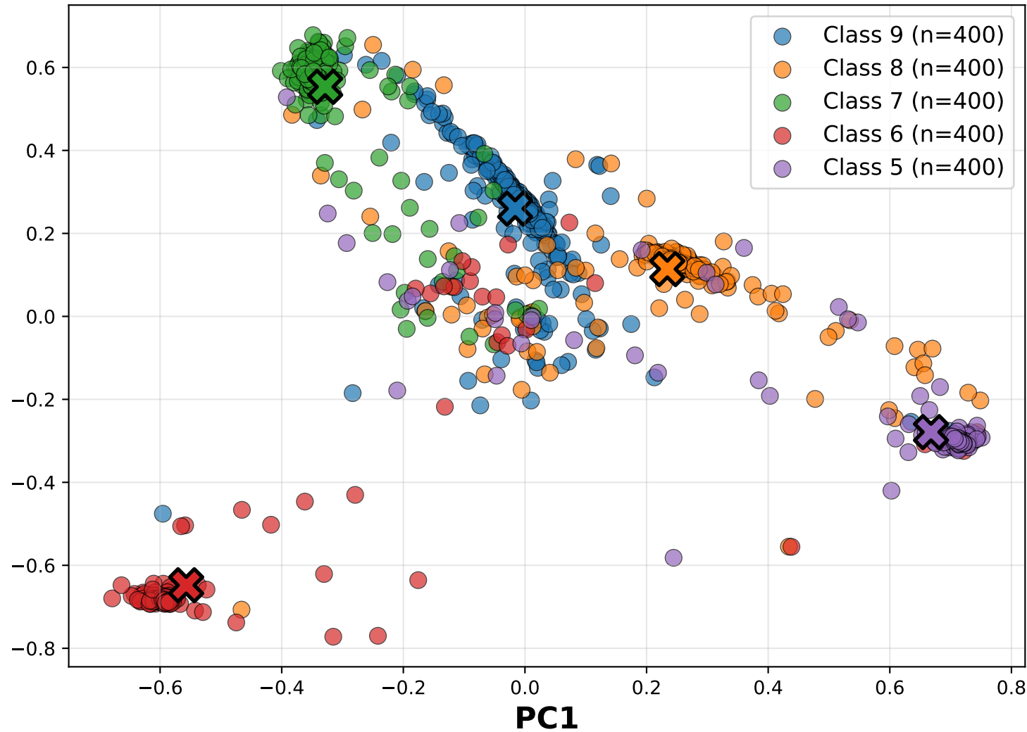
U_N : Rare Class Embeddings (Avg Intra-dist=0.093)
