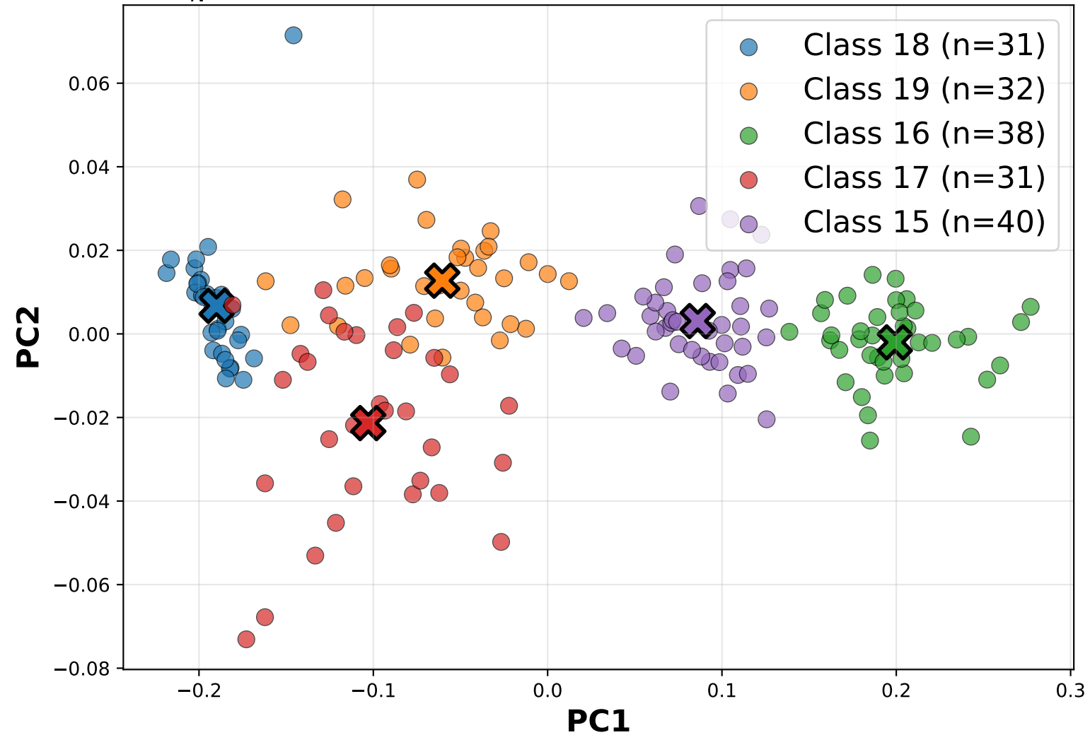
U_N^h : Rare Class Embeddings (Avg Intra-dist=0.029)
