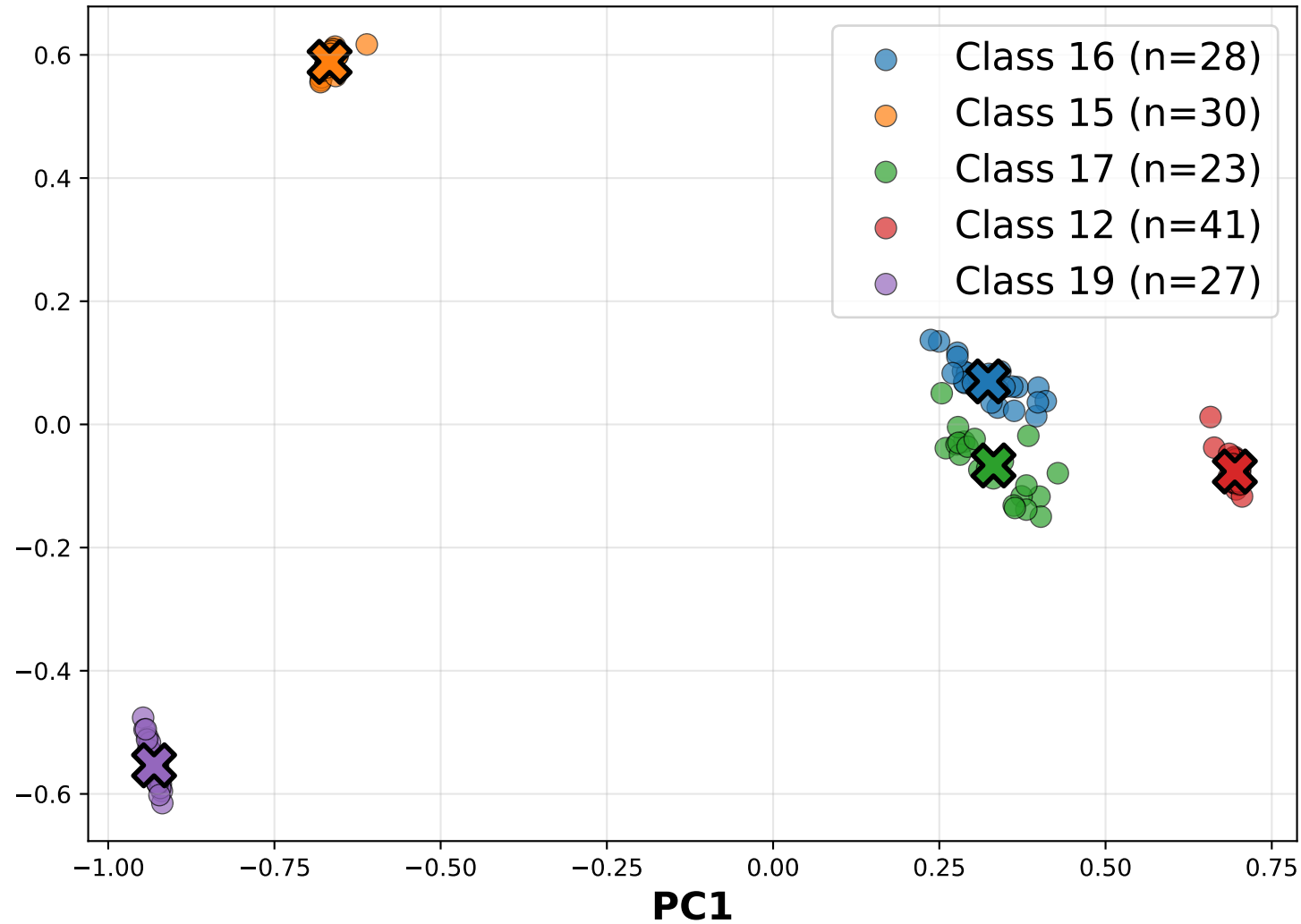
U_N : Rare Class Embeddings (Avg Intra-dist=0.035)
