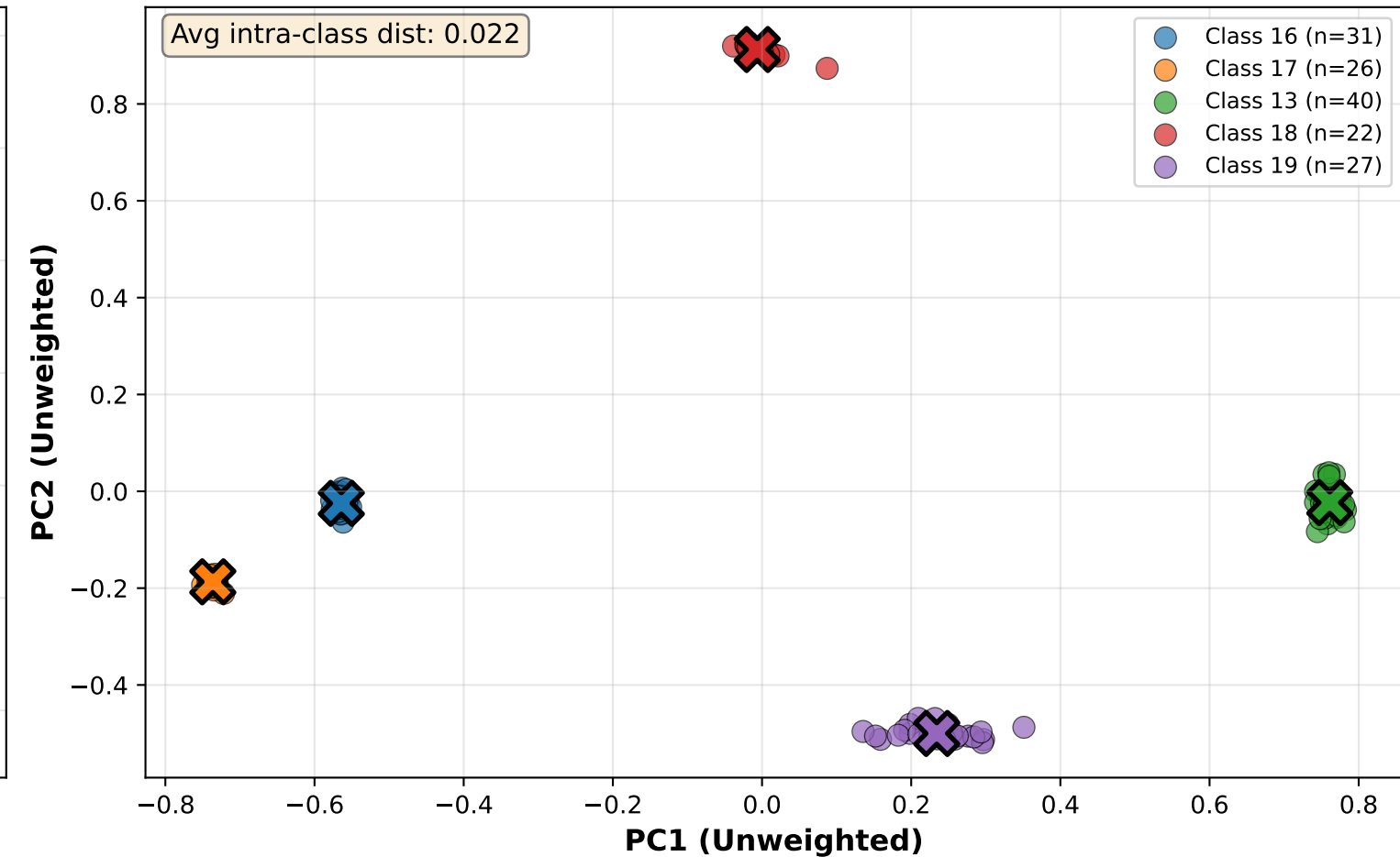
Unweighted U-Statistics: Rare Class Embeddings
