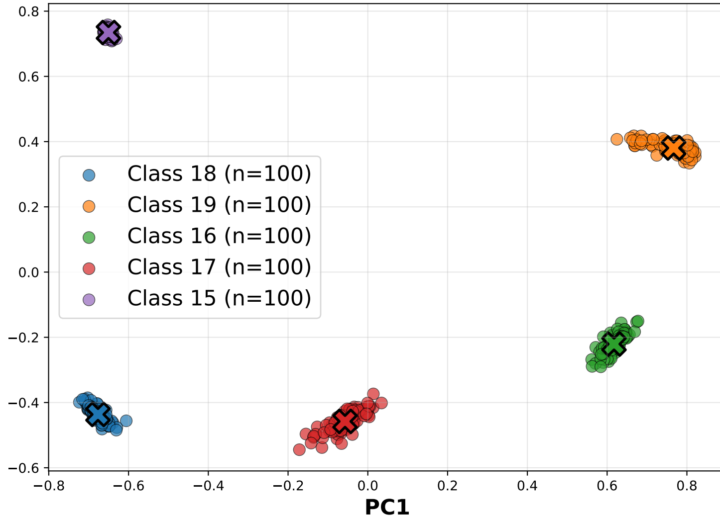
U_N : Rare Class Embeddings (Avg Intra-dist=0.030)
