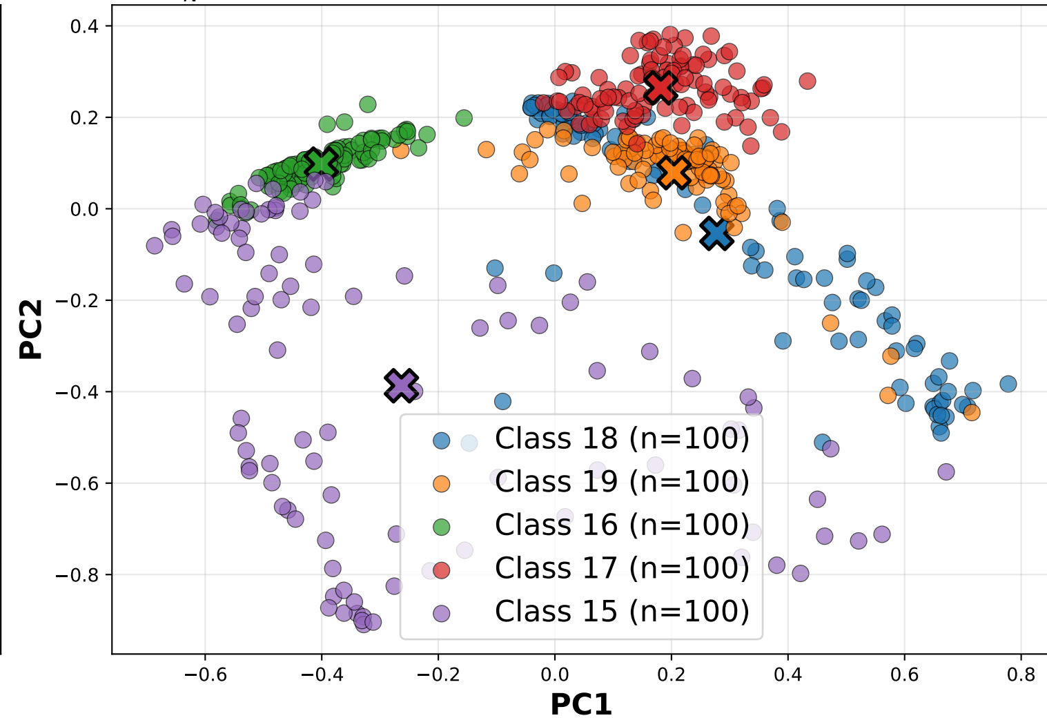
U_N^h : Rare Class Embeddings (Avg Intra-dist=0.217)
