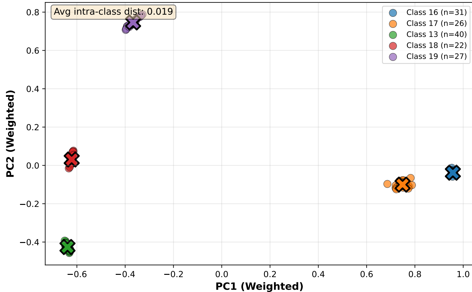
Weighted U-Statistics: Rare Class Embeddings
