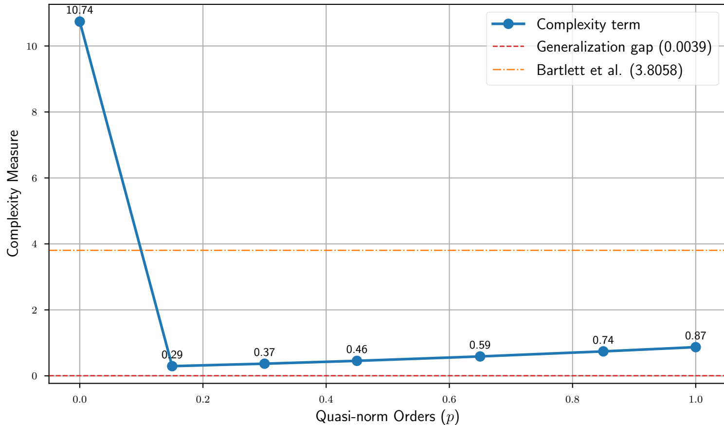
Effect of p on theoretical complexity
