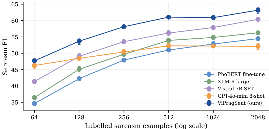
Low-resource sarcasm slice
