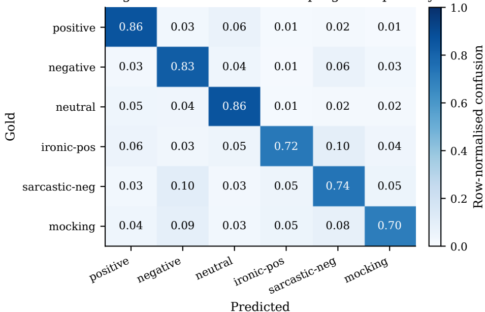
ViPragSent confusion matrix on pragmatic polarity
