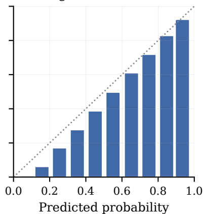
ViPragSent ECE=0.048
