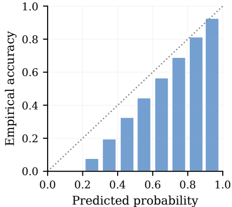
PhoBERT ECE=0.094
