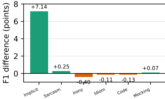
Figure 2: Per-label difference between ViPragSent-Final and the strongest best-tuned baseline result for each label. The zero line distinguishes positive margins from localized deficits; the vertical scale is not truncated to exaggerate small differences.
