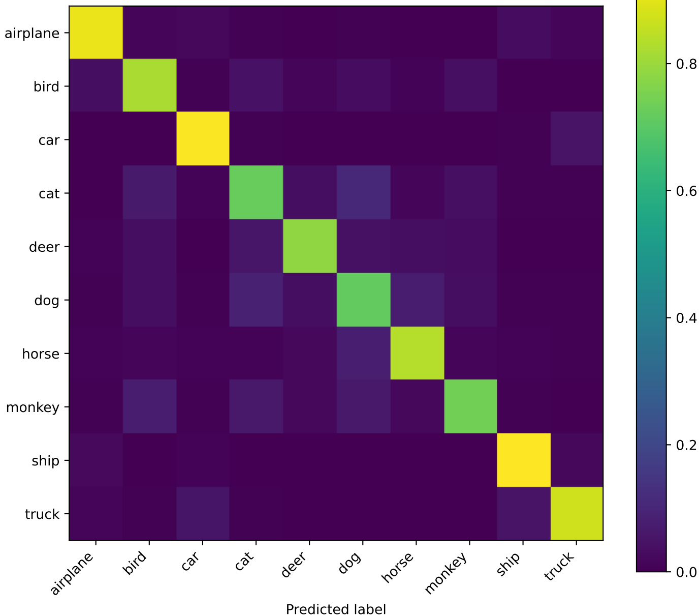
Fine-tuned ResNet50 normalized confusion matrix
