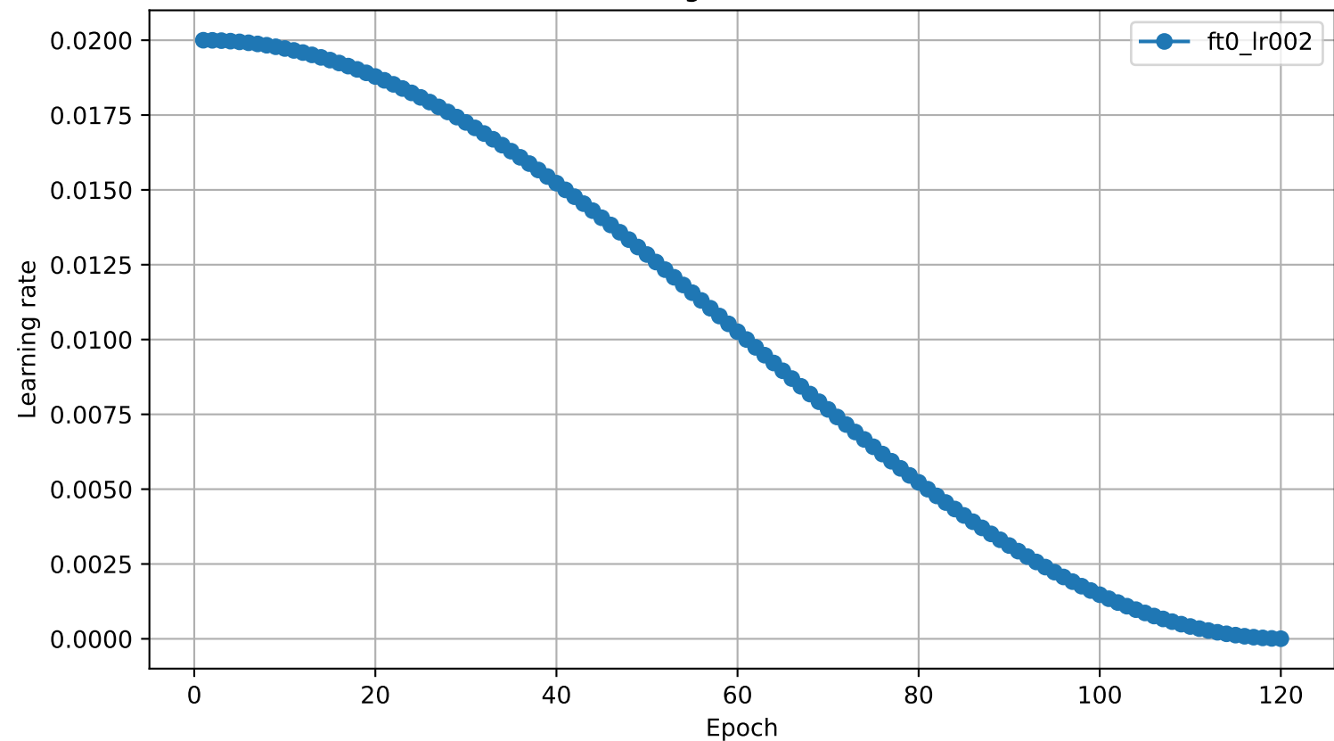
Learning-rate schedule
