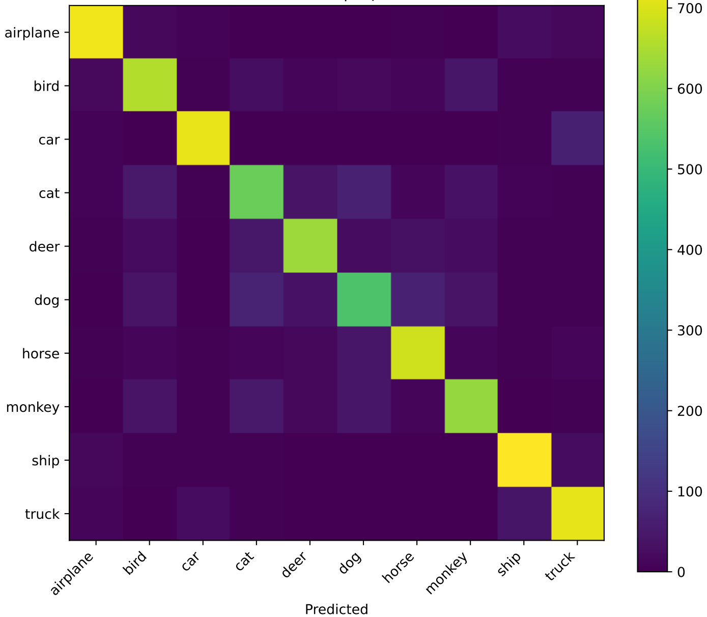
Confusion Matrix | Top-1=82.65%
