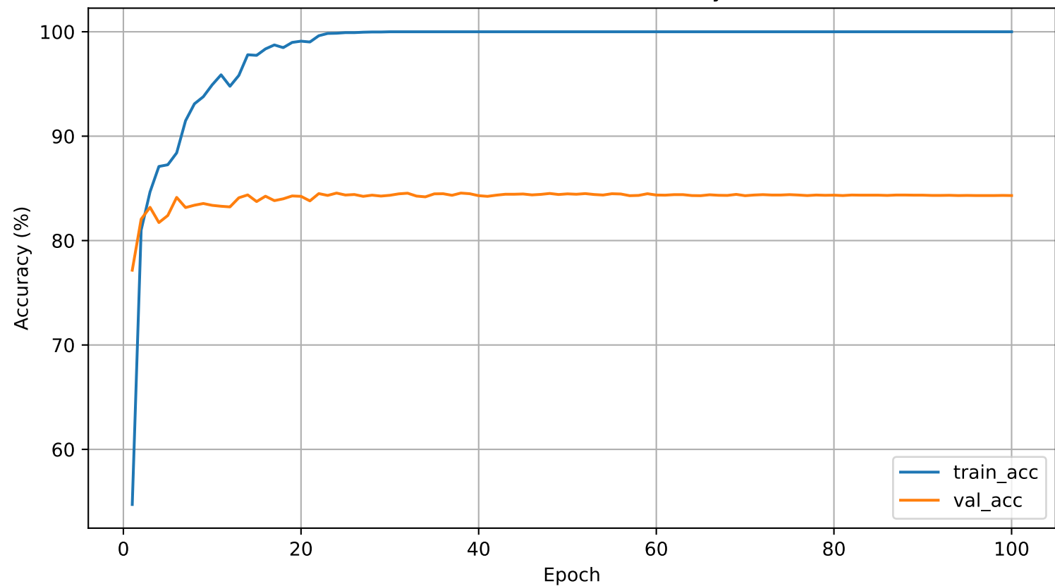
Linear Evaluation Accuracy
