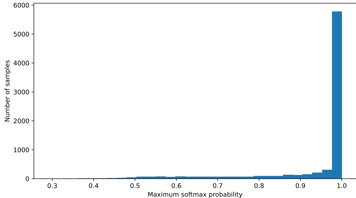
Linear Eval Confidence Distribution
