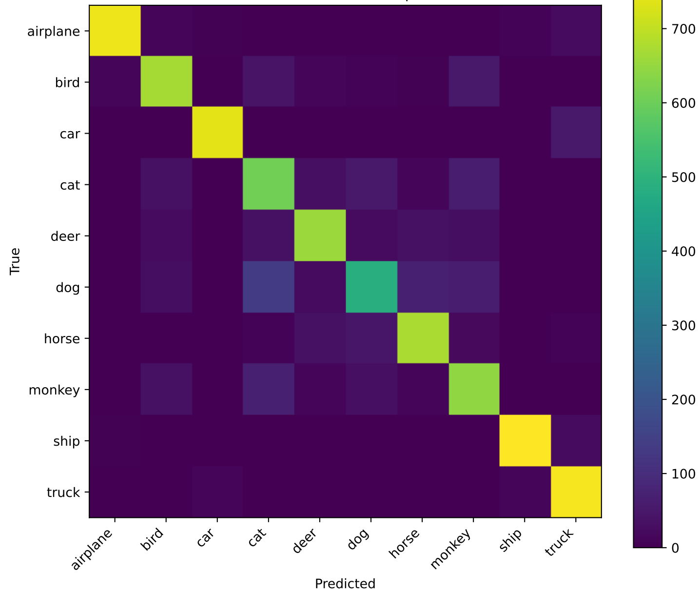
Linear Eval Confusion Matrix | Acc=84.55%
