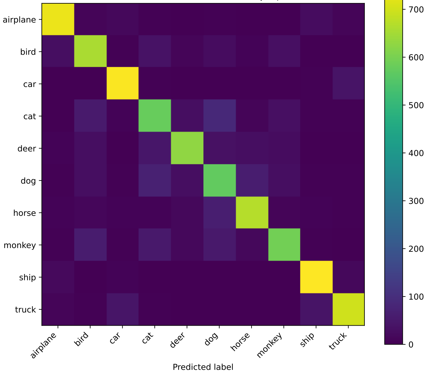
Fine-tuned ResNet50 confusion matrix | Top-1=82.70%
