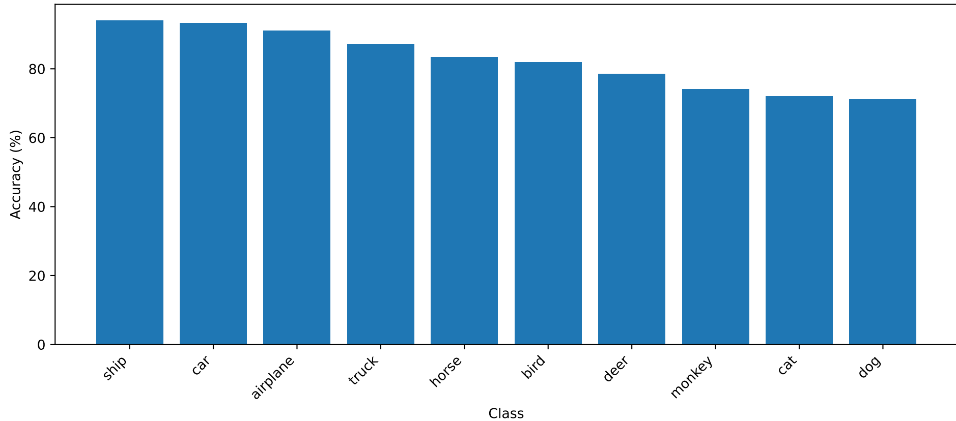
Fine-tuned ResNet50 per-class accuracy
