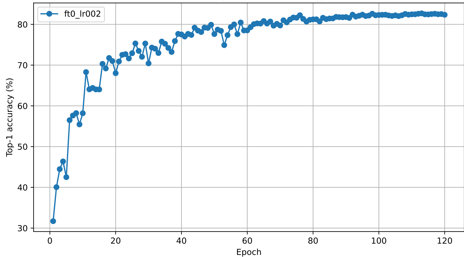
Fine-tuning validation accuracy
