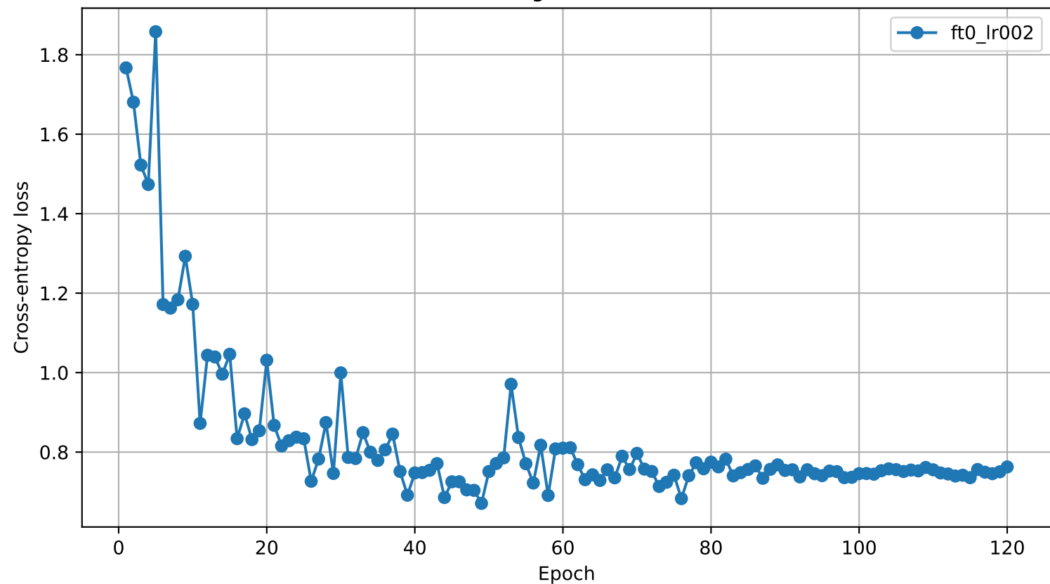
Fine-tuning validation loss
