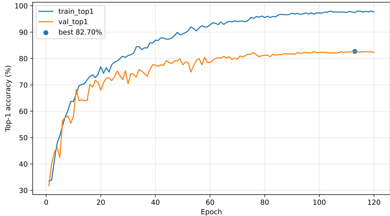
Fine-tuning accuracy curves
