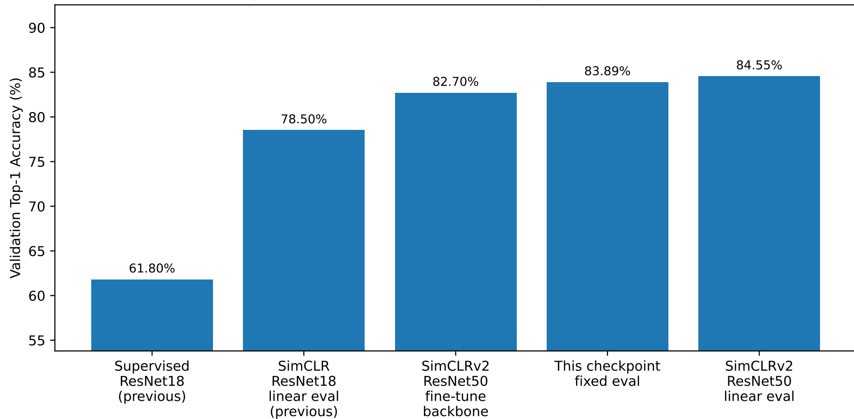
Comparison of downstream evaluation protocols on STL-10
