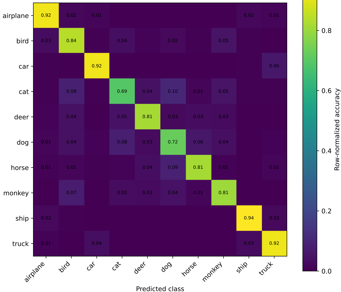
Fine-tuned SimCLRv2 ResNet50 normalized confusion matrix
