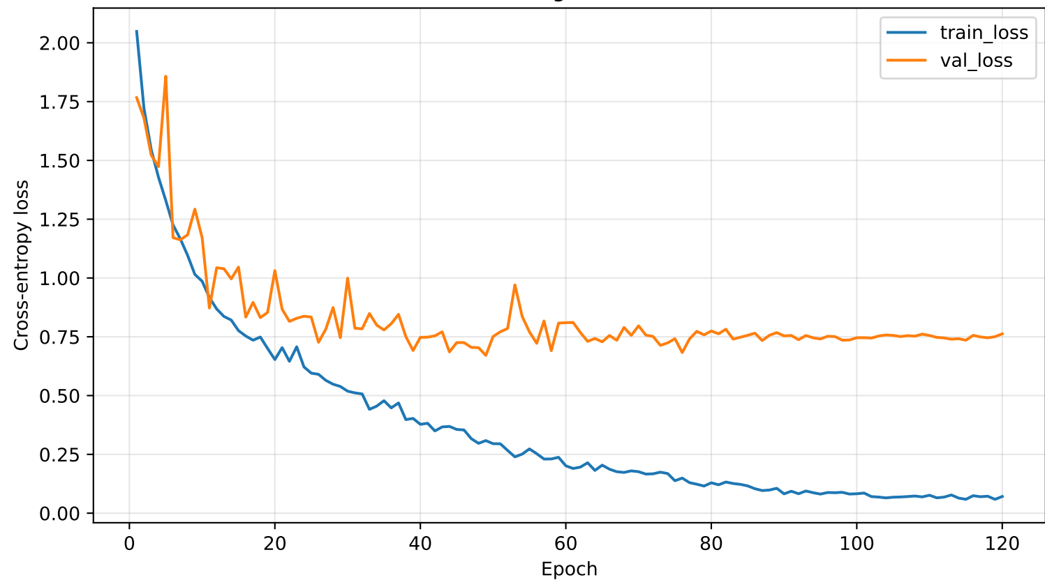
Fine-tuning loss curves
