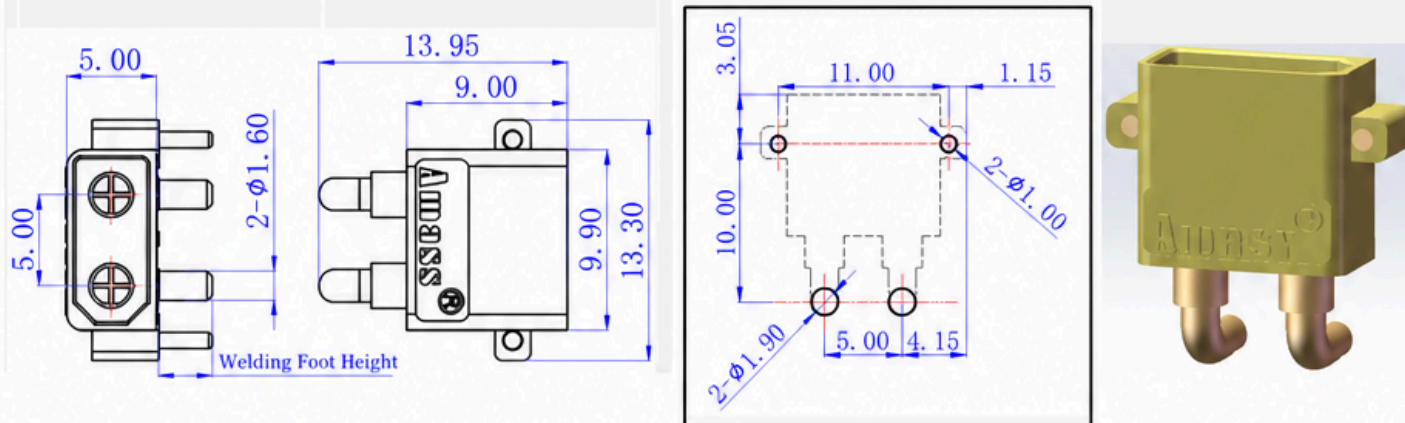
Installation Hole Diagram
