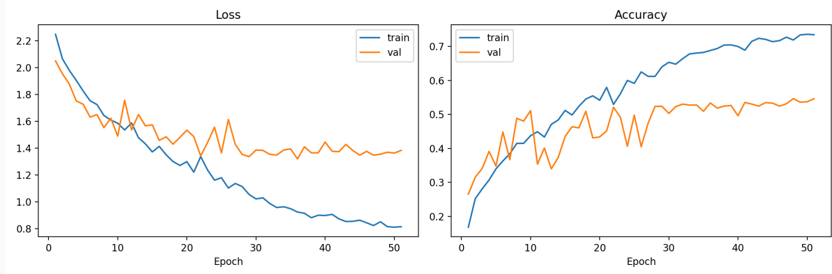
Figure 40: Training curves for mel LSTM.
