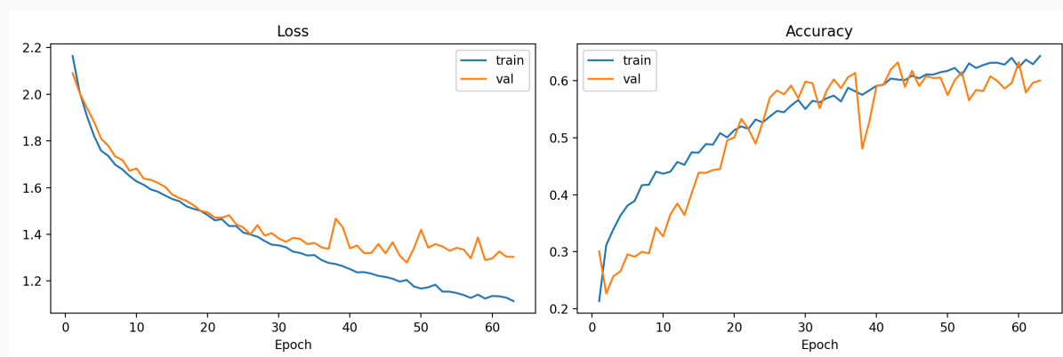
Figure 39: Training curves for mel CNN.
