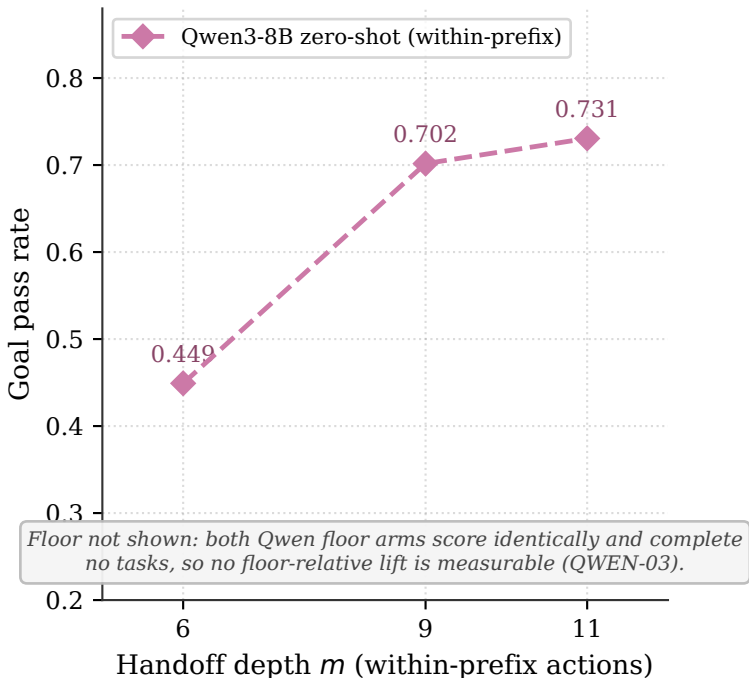
Within-prefix depth curve (Second executor family: Qwen3-8B)
