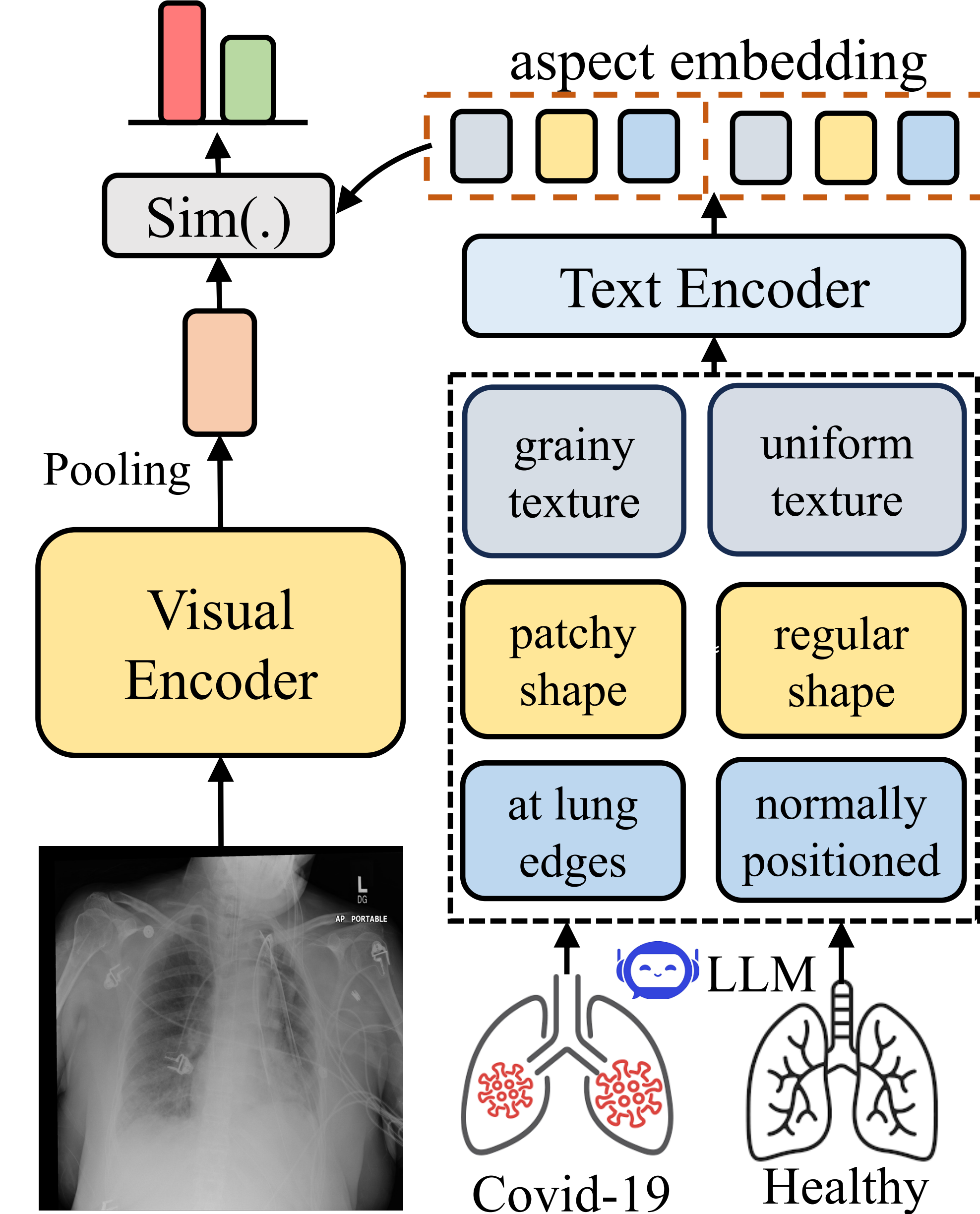
B) Contrastive head for inferring unseen diseases
