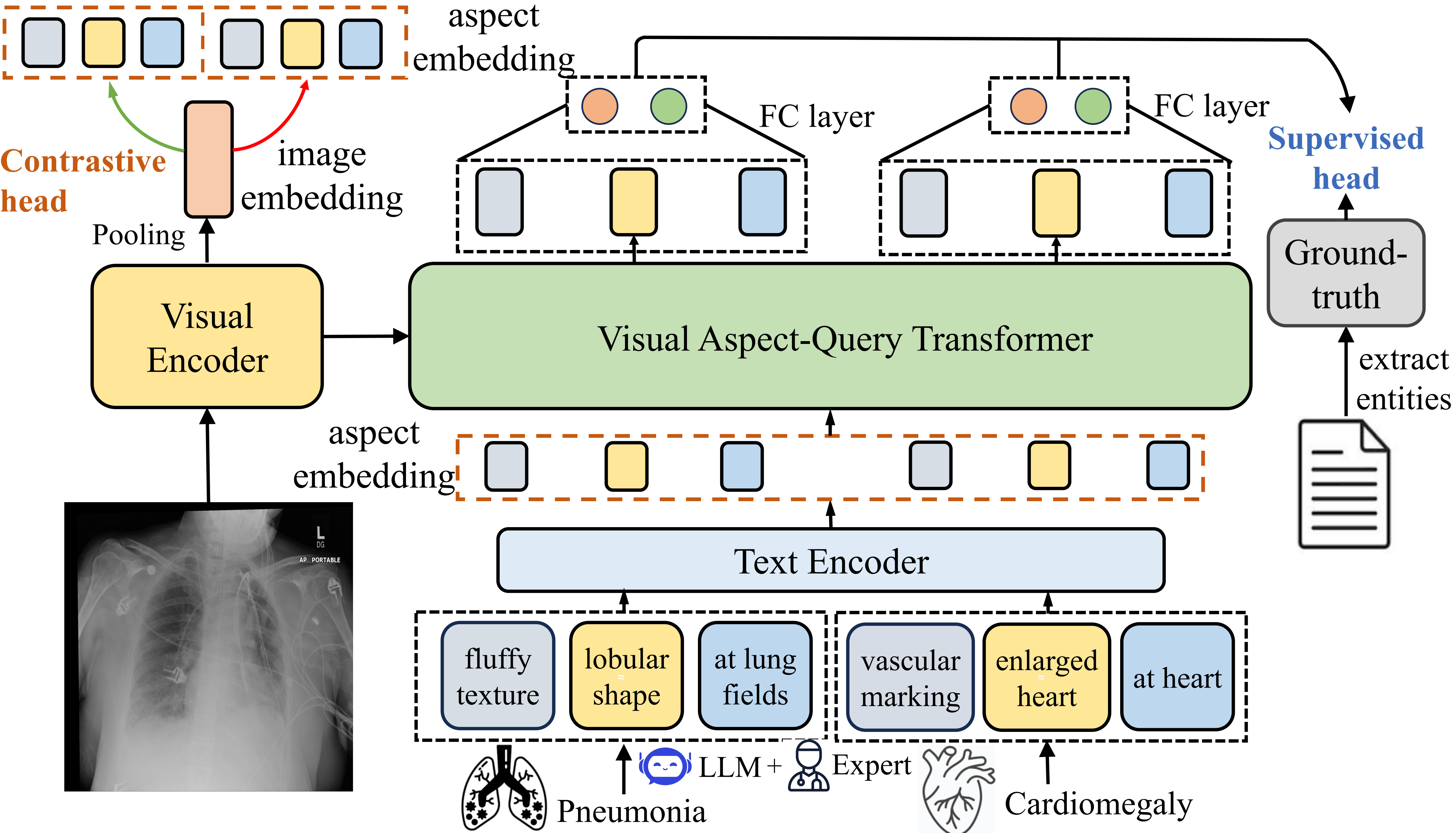
A) Aspect-oriented dual-head Transformer
