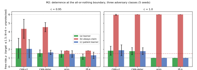
Fig. 12: Deterrence at the all-or-nothing boundary, three adversary classes. Scripted commitment (grim / tit-for-tat on observed claim rates) holds best-response and 3\times -budget patient learners at exactly \rho=1.0 ; league-learned policies (either credit horizon) leave \rho \approx 1.8 . Always-claim hits the Prop. 1 boundary ( \rho \rightarrow N ) for every policy—with D=1 efficiency collapsing, i.e. levelling-down, not profit. Patience never pays.
