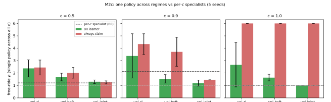
Fig. 13: One policy across regimes: a single c -conditioned policy trained by multi- c league RL with a grim-teacher auxiliary loss (uni-joint) matches the per- c specialists against trained best responses and holds the committed claimer far below them at c \leq 0.9 ; without the teacher (uni-rl) commitment never emerges, and with teaching only at initialization (uni-bcft) it erodes.
