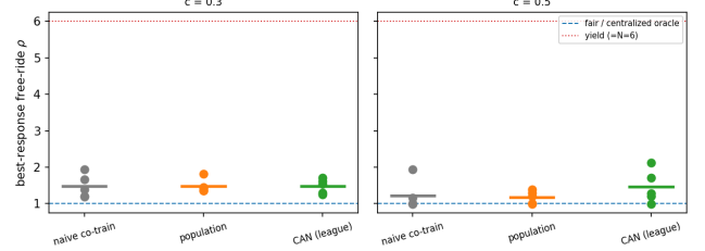
Fig. 6: Per-seed best-response \rho for three adversarial training schemes (5 seeds). The schemes are indistinguishable (all \rho \approx 1.2 – 1.5 ); what matters is training against a learned exploiter rather than a static one. The dotted line marks the all-yield ceiling ( \rho=N ).
