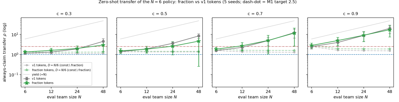
Fig. 9: The transfer fragility is the lone defector, not team size. Solid: lone-defector ( D=1 ) zero-shot transfer of the N=6 policy, v1 vs N -invariant fraction tokens—both degrade toward the all-yield line as N grows at high c . Dashed: the same policies at constant defector fraction ( D=N/6 ) transfer essentially perfectly at every c . Log-log; dash-dot line marks \rho=2.5 .
