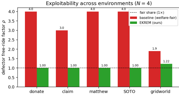
Fig. 2: Defector free-ride factor \rho per environment ( N=4 ). A single self-interested agent free-rides 1.9–4 \times against the welfare-fair baseline; EKREM brings every case back toward the fair share ( \rho \approx 1 ).
