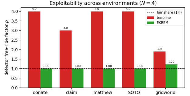
Fig. 2: Defector free-ride factor \rho per environment ( N=4 ). A single self-interested agent free-rides 1.9\text{--}4\times against the welfare-fair baseline; EKREM brings every case back toward the fair share ( \rho \approx 1 ).
