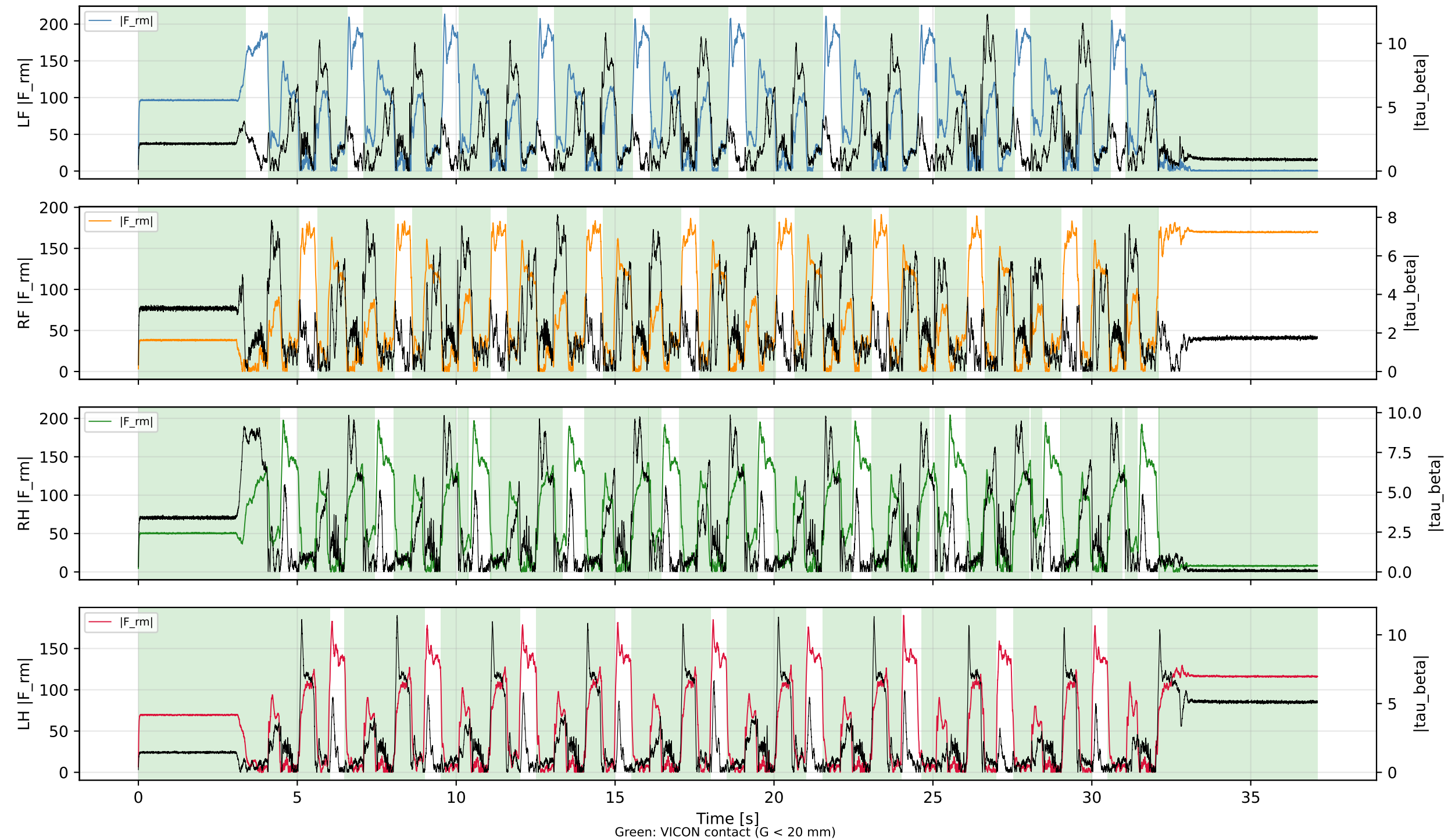
GMO Residuals vs VICON Ground Truth — FLAT_WLW_NEW_REAL_3
