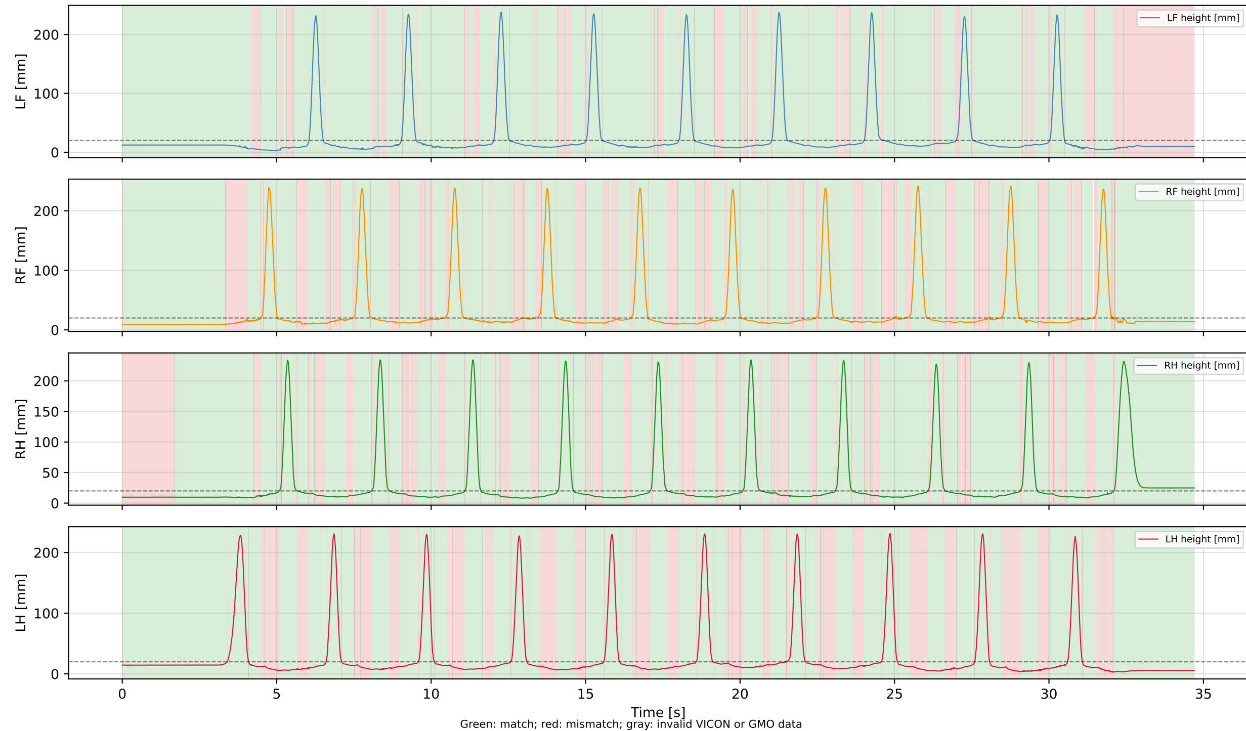
Contact Detection — FLAT_WLW_NEW_REAL_4 (VICON < 20 mm; F_rm 50/25, tau_beta 3.00/1.50)
