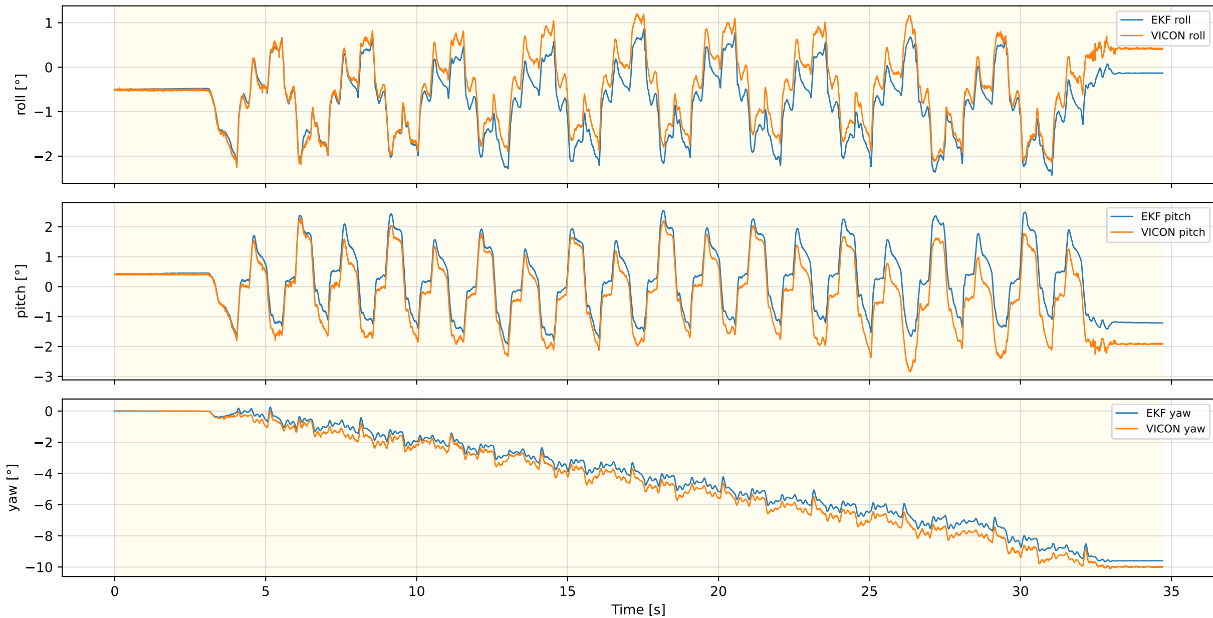
Inner EKF Attitude — FLAT_WLW_NEW_REAL_4
