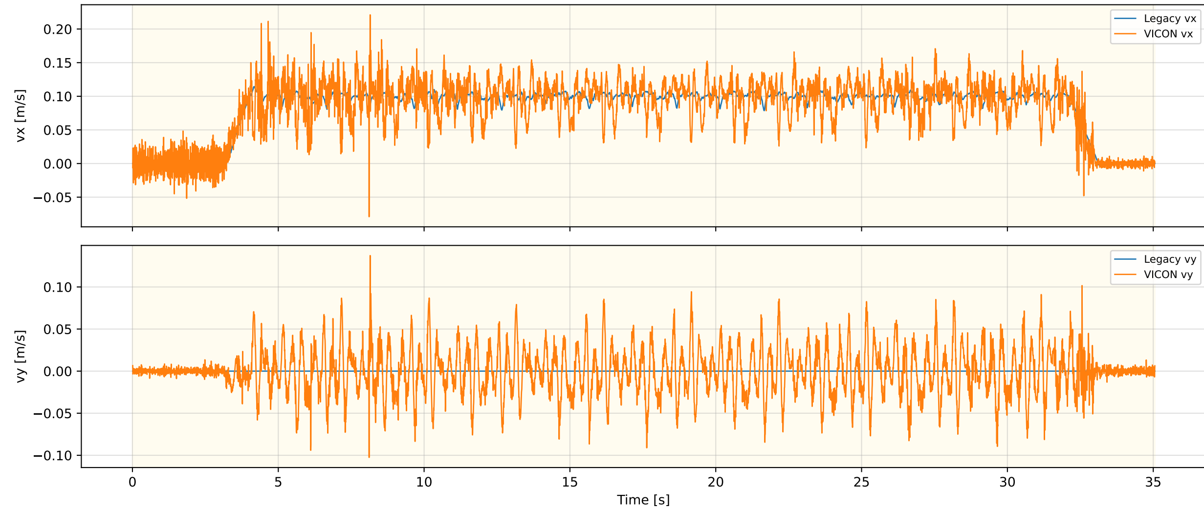
Legacy Odometry Velocity — FLAT_WLW_OLD_REAL_2
