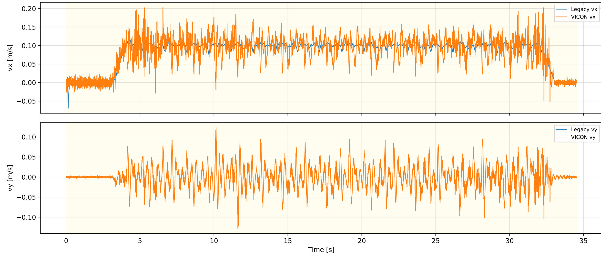
Legacy Odometry Velocity — FLAT_WLW_OLD_REAL_5
