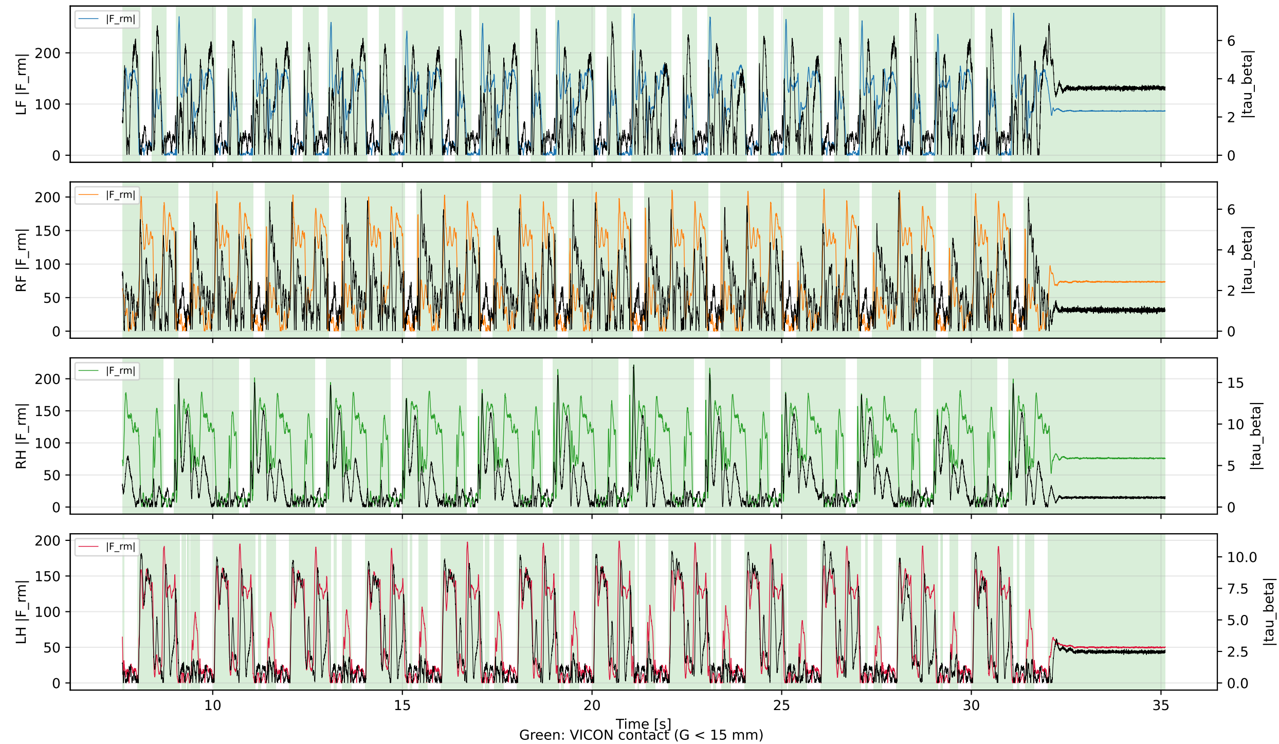
GMO Residuals vs VICON Ground Truth — FLAT_Walk_NEW_REAL_1
