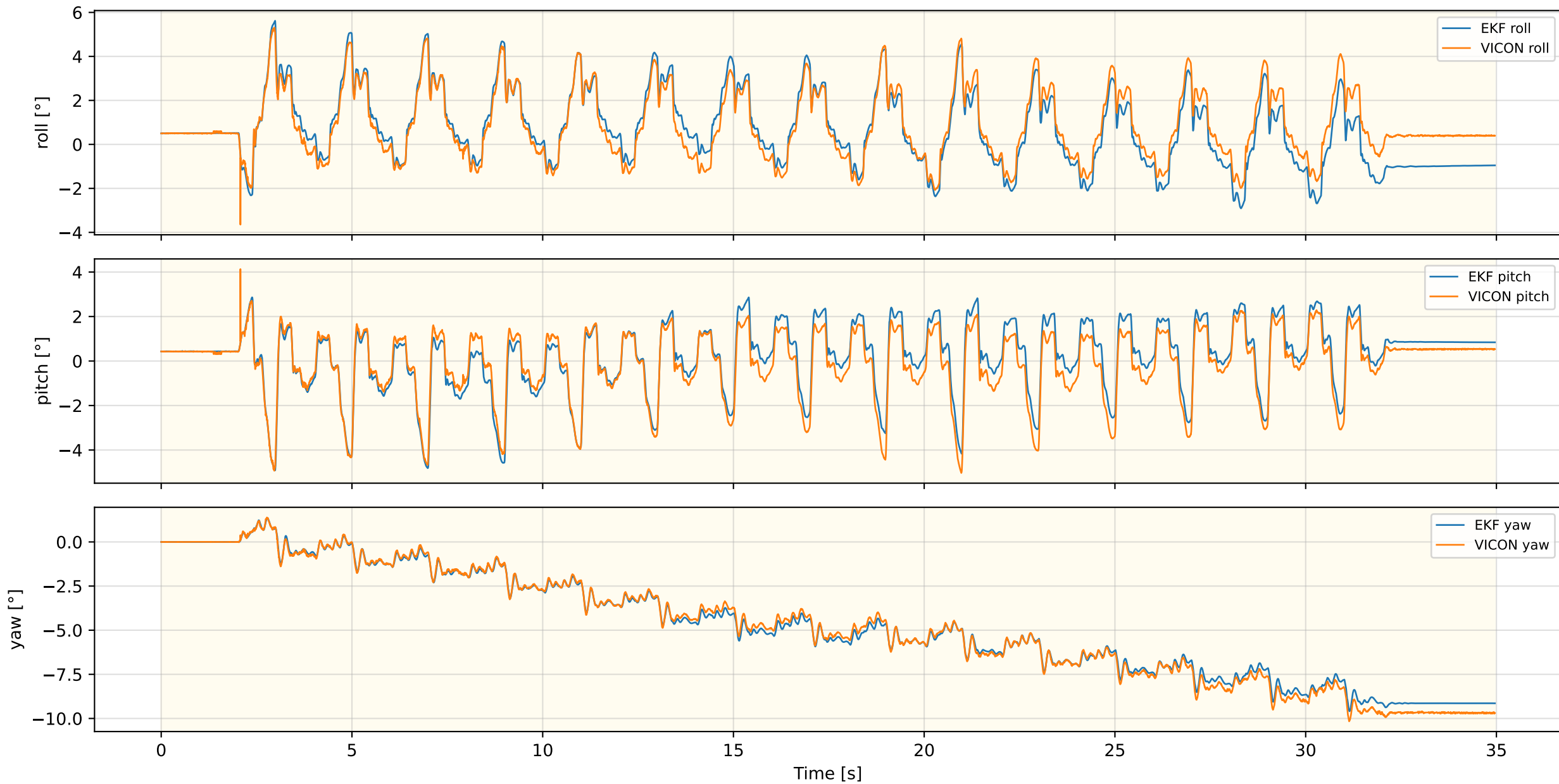
Inner EKF Attitude — FLAT_Walk_NEW_REAL_4
