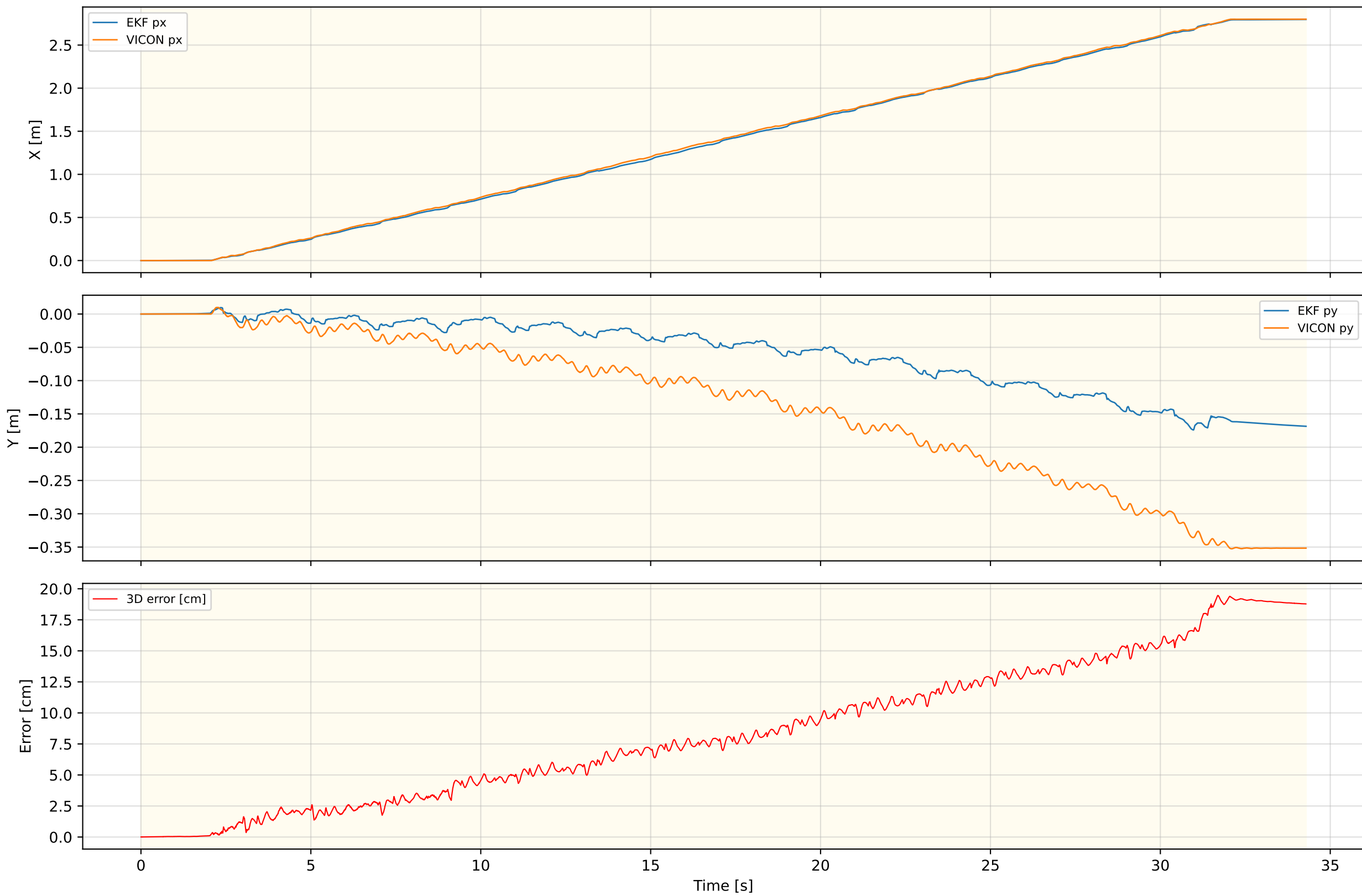
Inner EKF Position — FLAT_Walk_NEW_REAL_5
