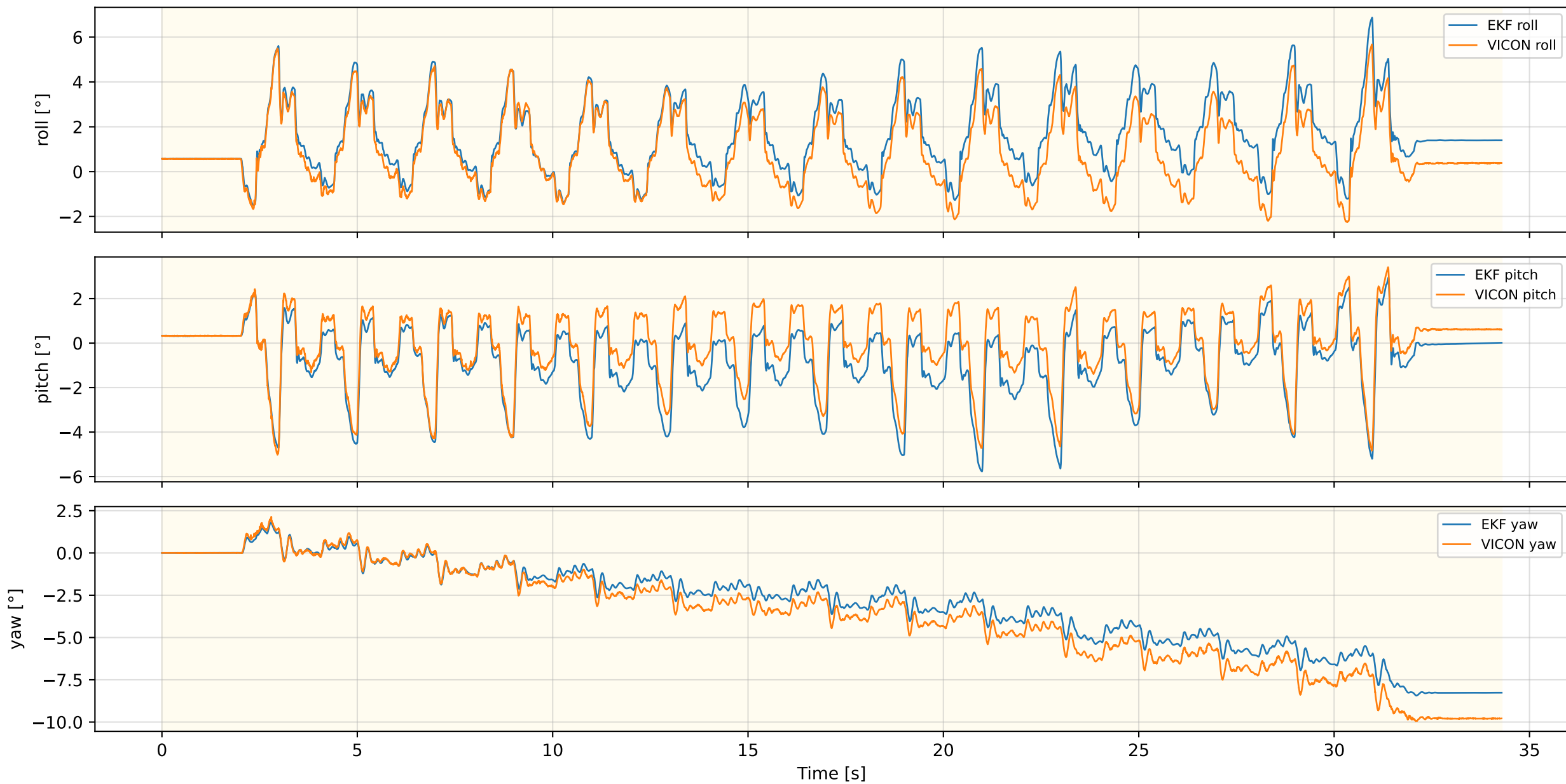
Inner EKF Attitude — FLAT_Walk_NEW_REAL_5
