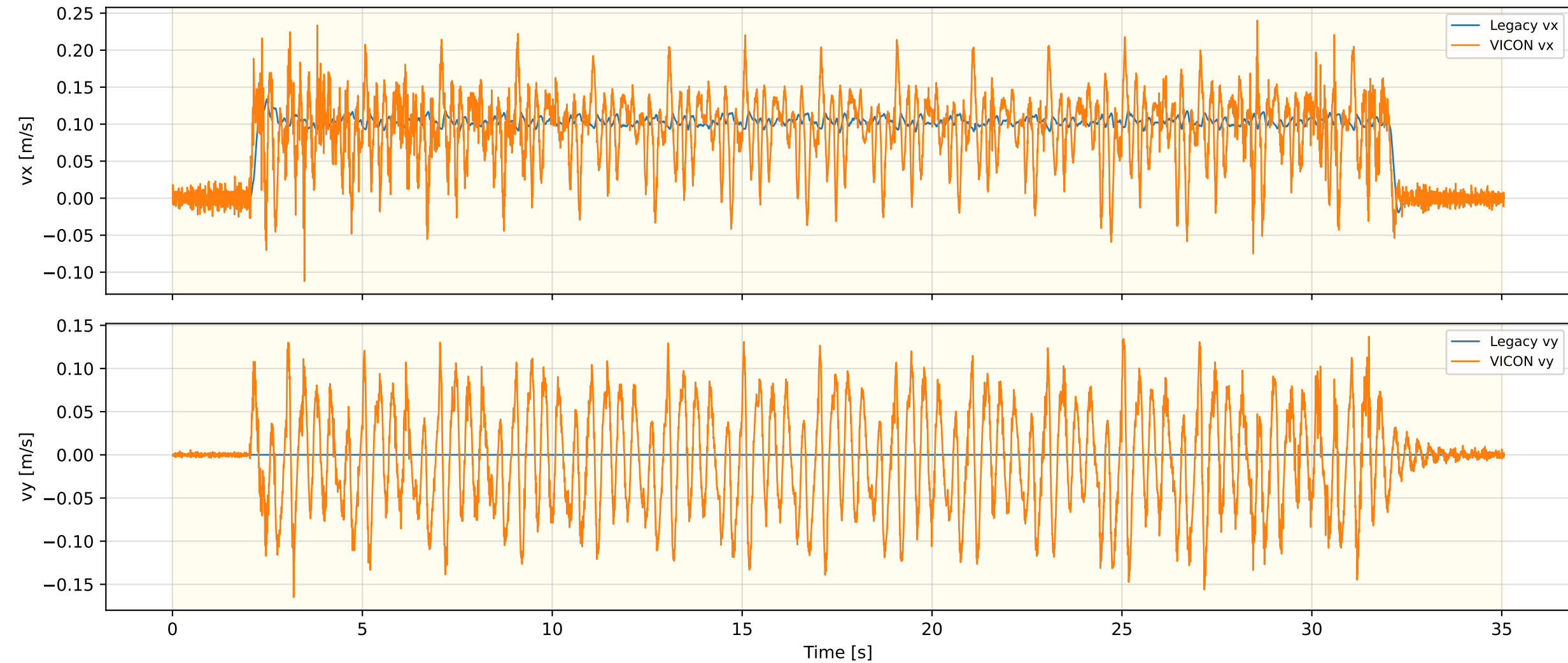
Legacy Odometry Velocity — FLAT_Walk_OLD_REAL_1
