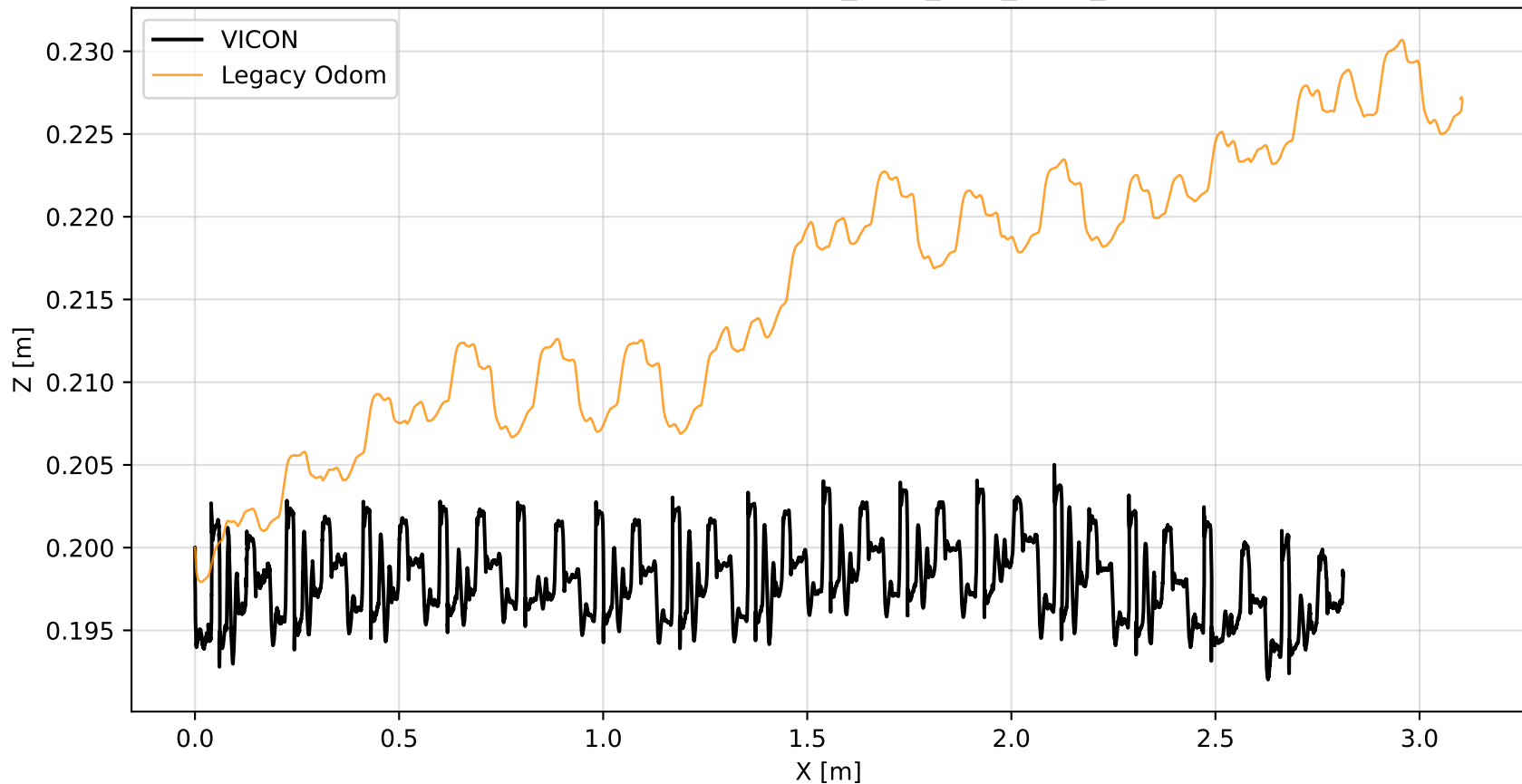
XZ Trajectory — FLAT_Walk_OLD_REAL_1
