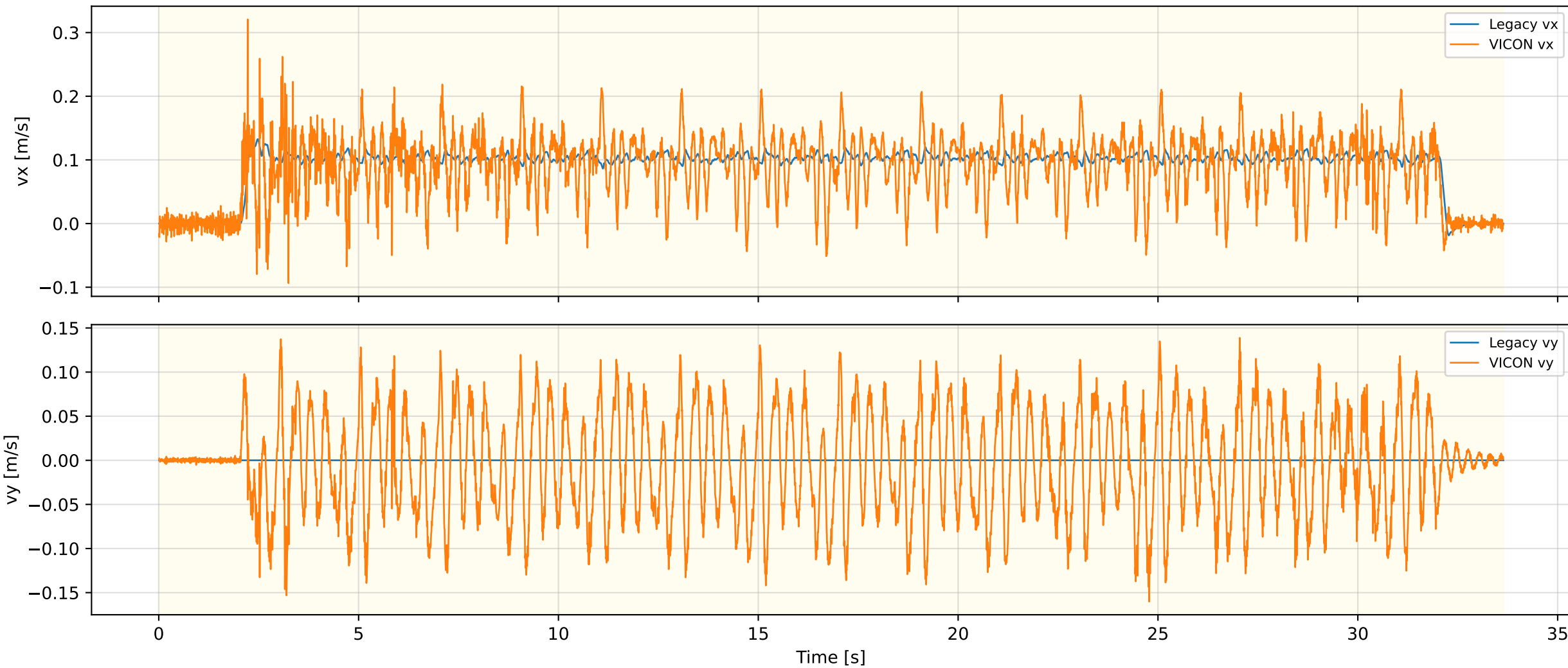
Legacy Odometry Velocity — FLAT_Walk_OLD_REAL_4
