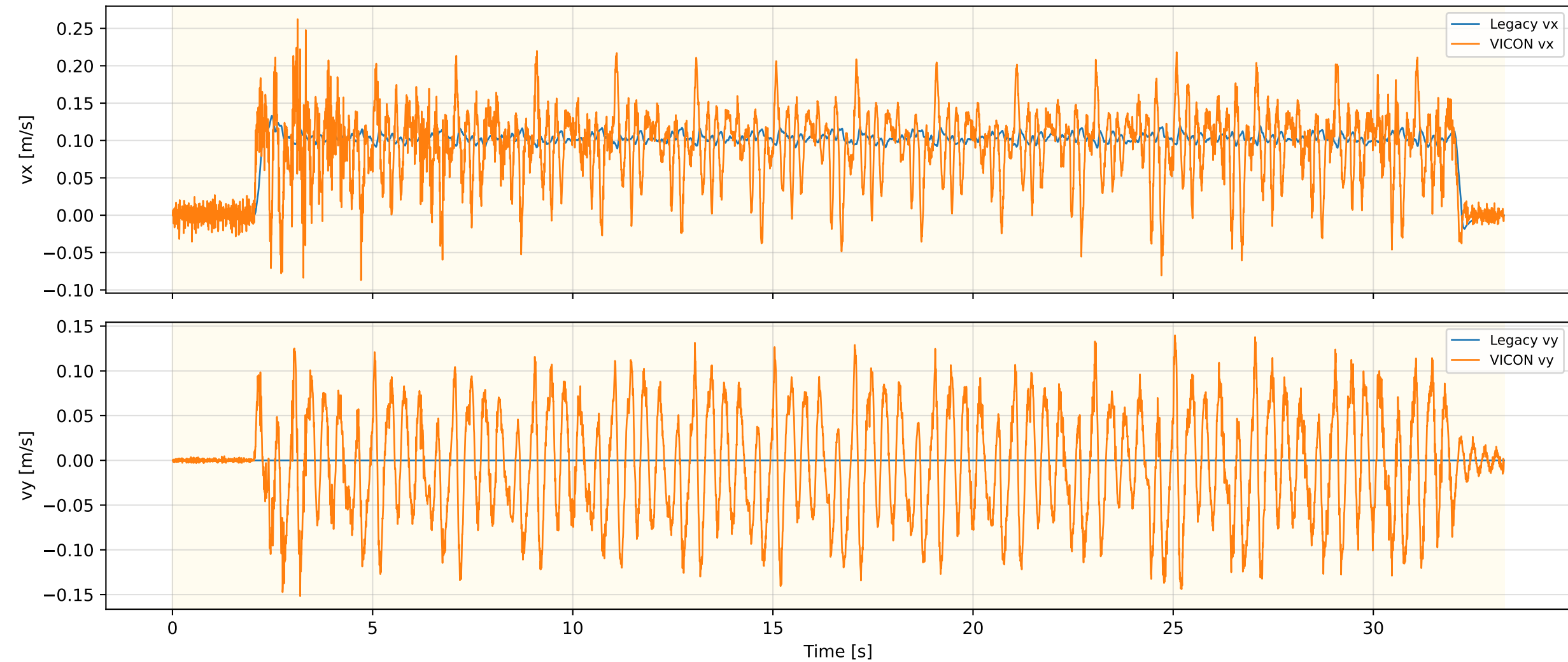
Legacy Odometry Velocity — FLAT_Walk_OLD_REAL_5
